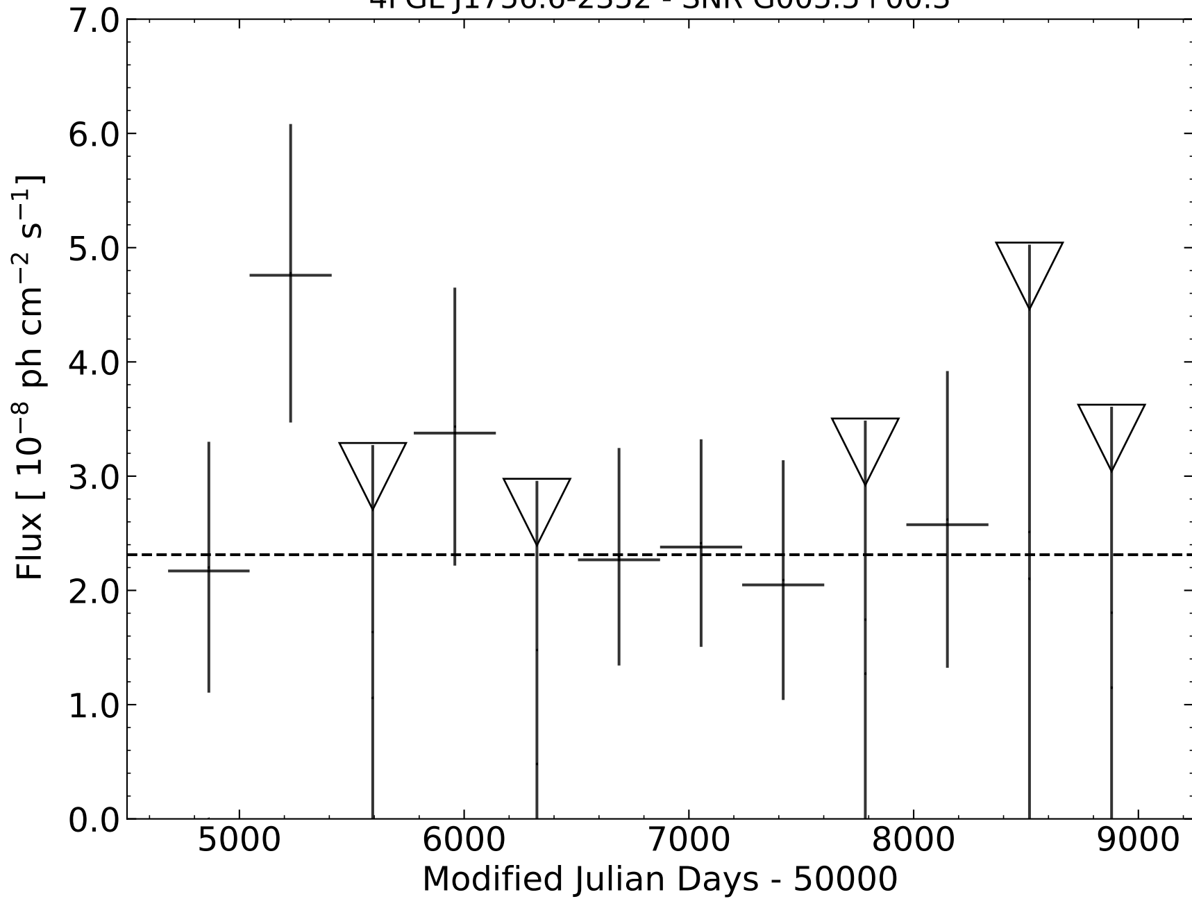
4FGL J1756.6-2352 - SNR G005.5+00.3
