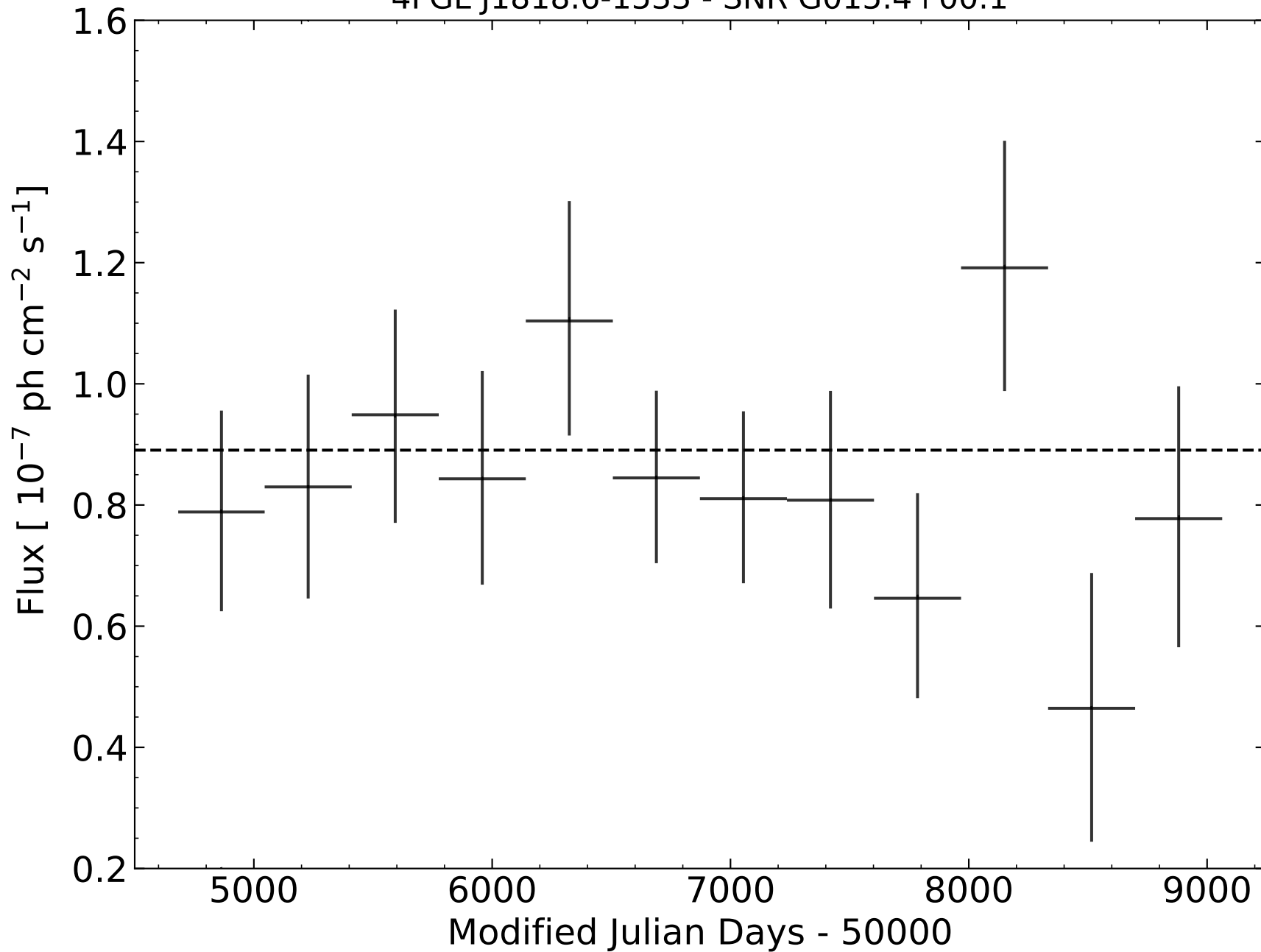
4FGL J1818.6-1533 - SNR G015.4+00.1
