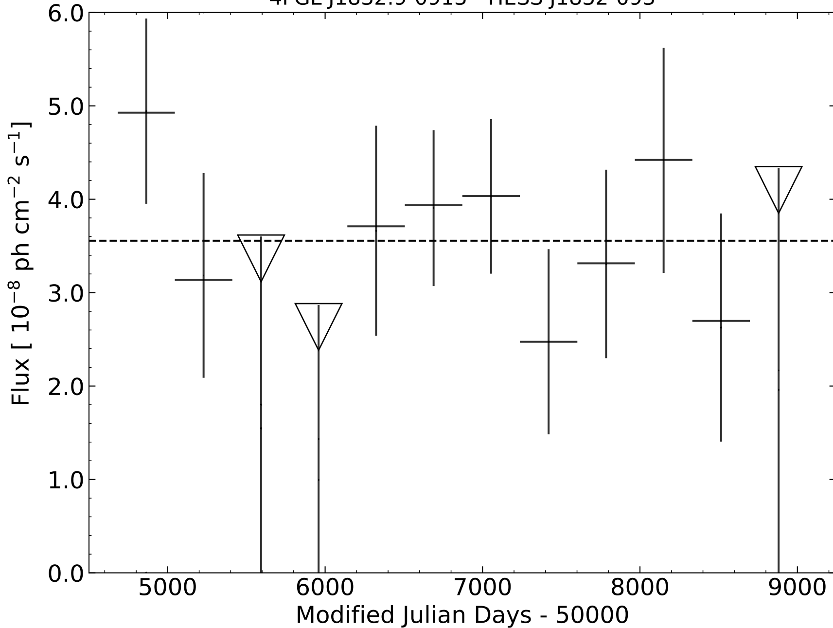
4FGL J1832.9-0913 - HESS J1832-093
