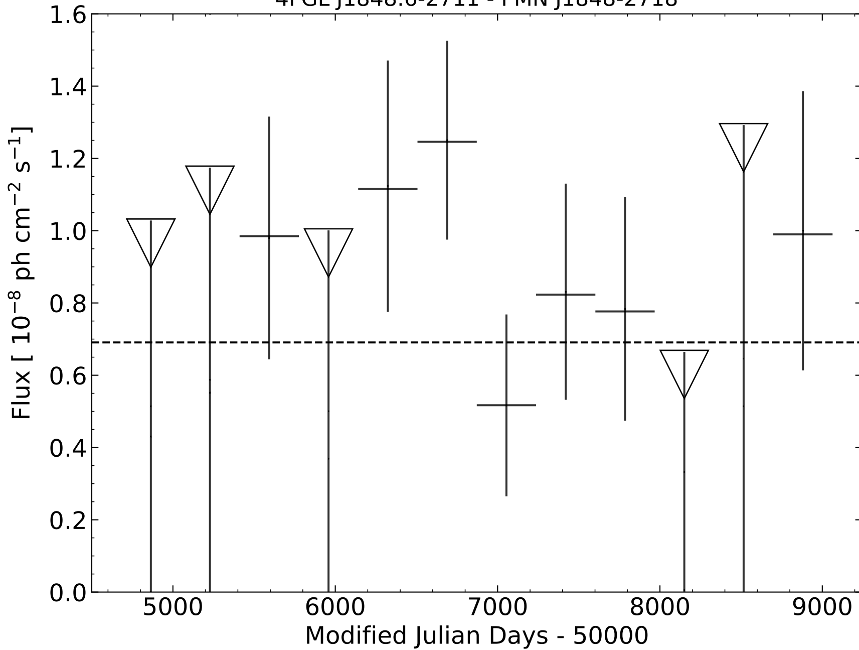
4FGL J1848.6-2711 - PMN J1848-2718
