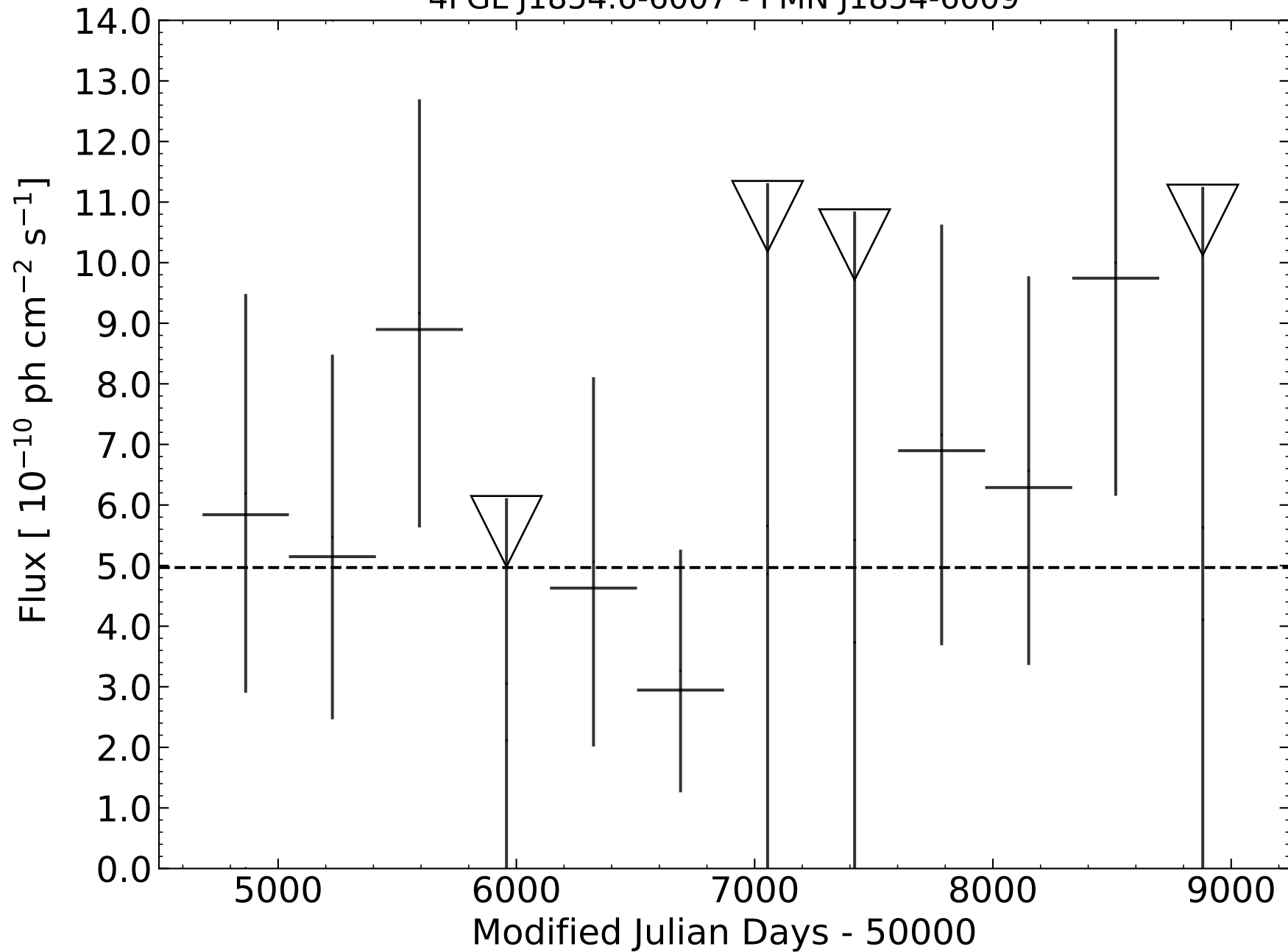
4FGL J1854.6-6007 - PMN J1854-6009
