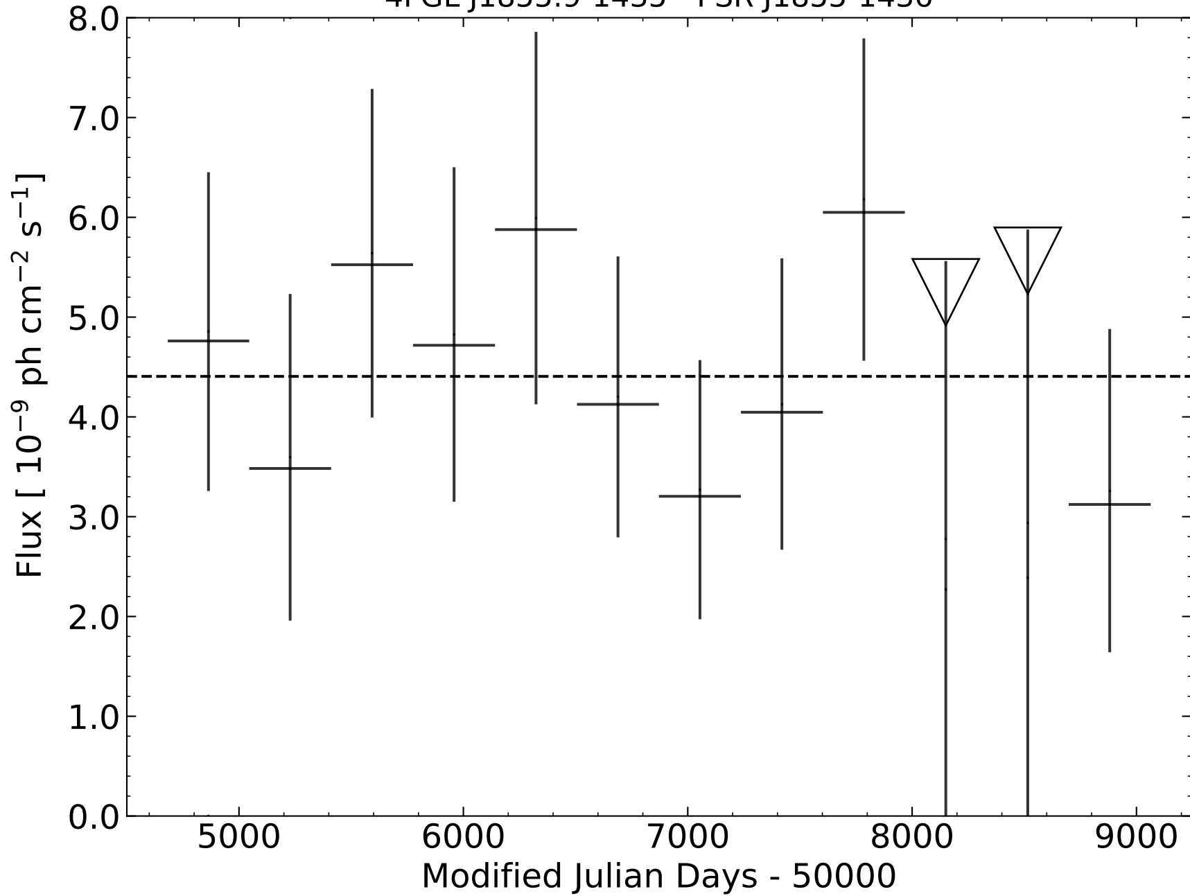
4FGL J1855.9-1435 - PSR J1855-1436
