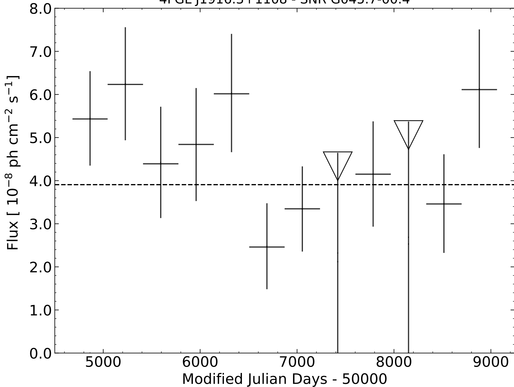
4FGL J1916.3+1108 - SNR G045.7-00.4
