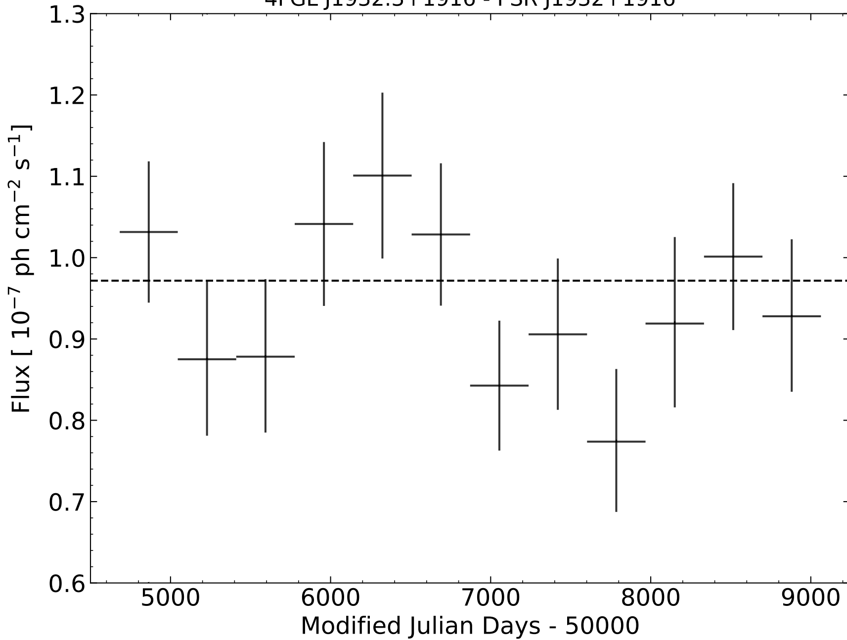
4FGL J1932.3+1916 - PSR J1932+1916
