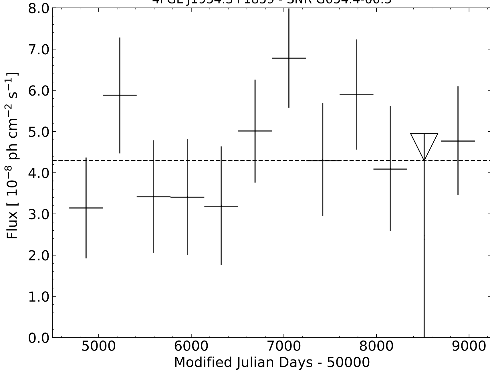
4FGL J1934.3+1859 - SNR G054.4-00.3
