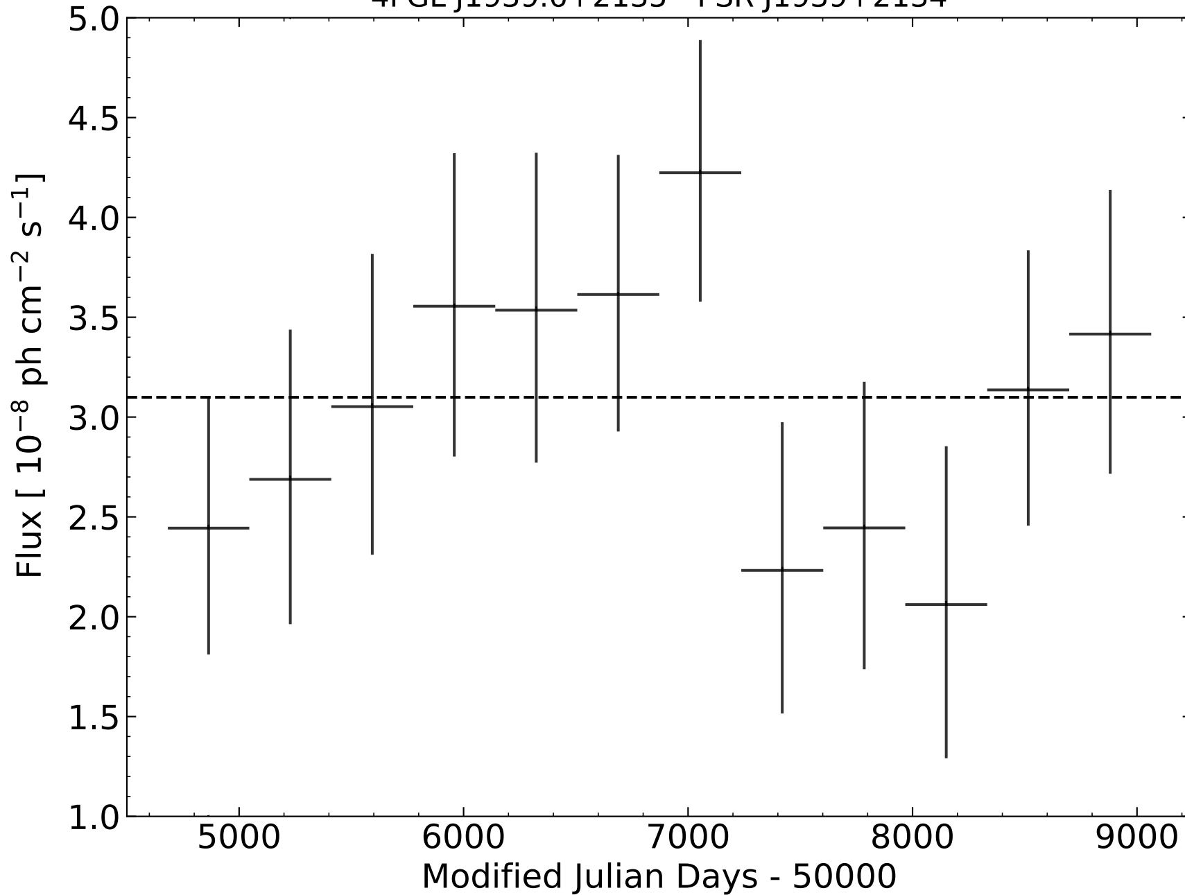
4FGL J1939.6+2135 - PSR J1939+2134
