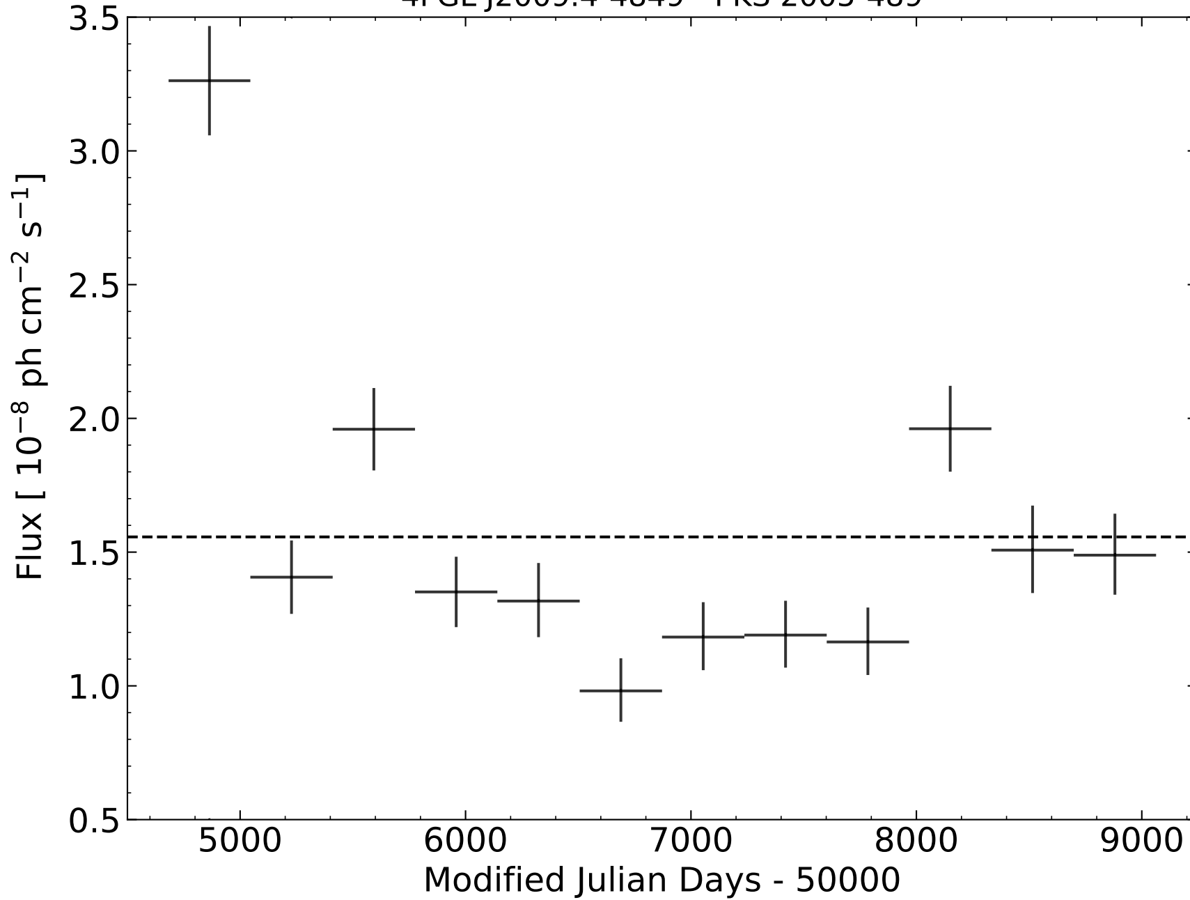
4FGL J2009.4-4849 - PKS 2005-489
