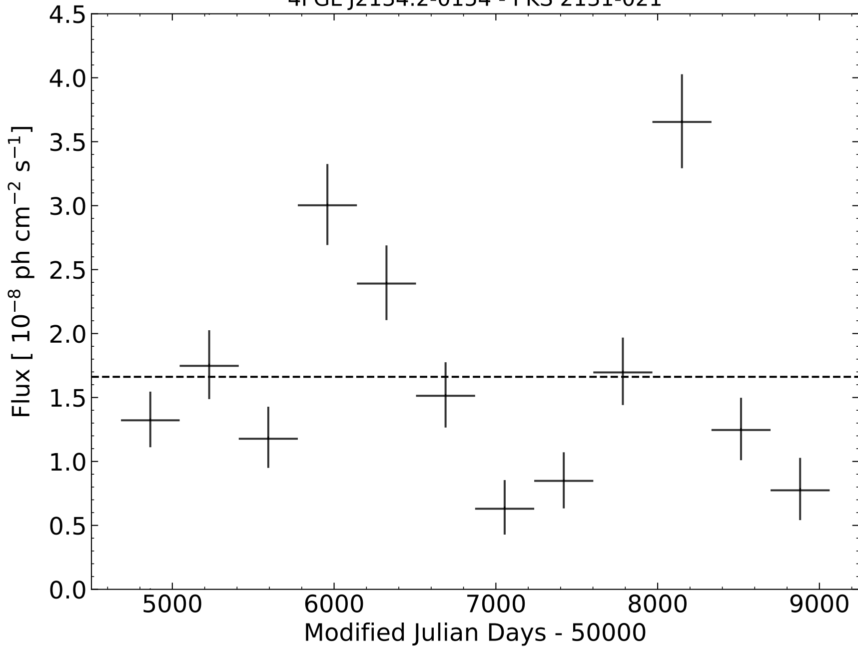
4FGL J2134.2-0154 - PKS 2131-021
