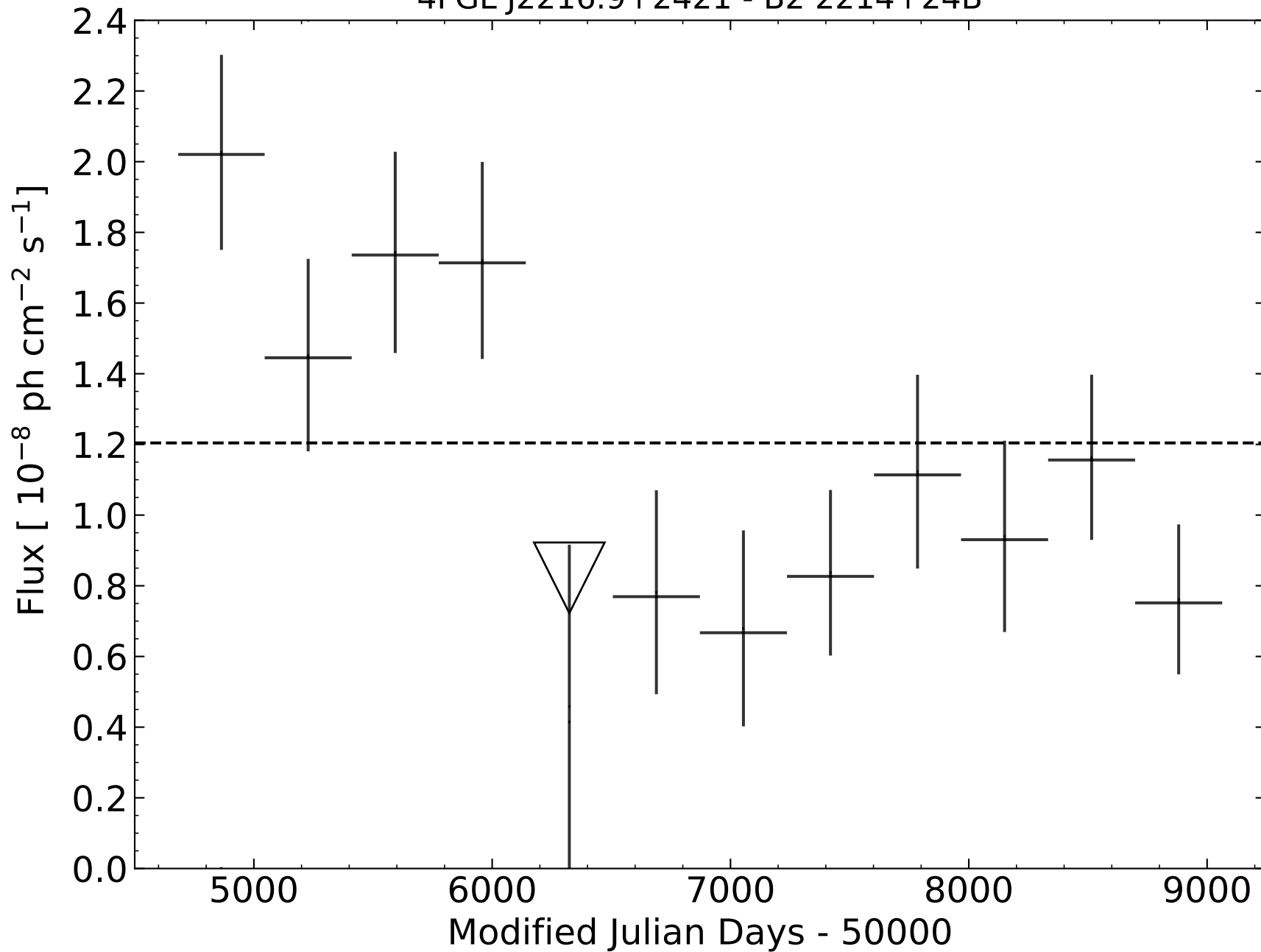
4FGL J2216.9+2421 - B2 2214+24B
