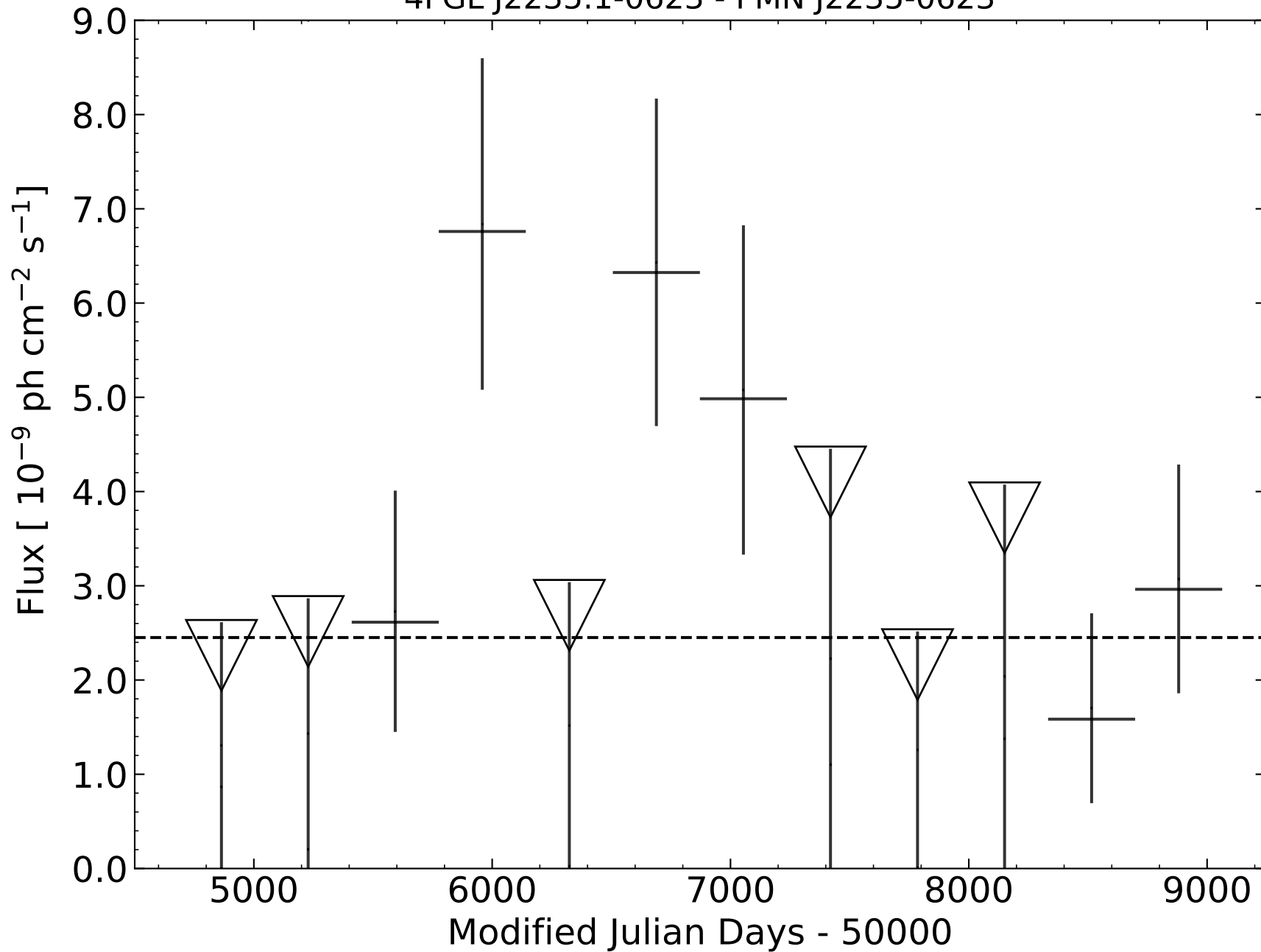
4FGL J2235.1-0623 - PMN J2235-0623
