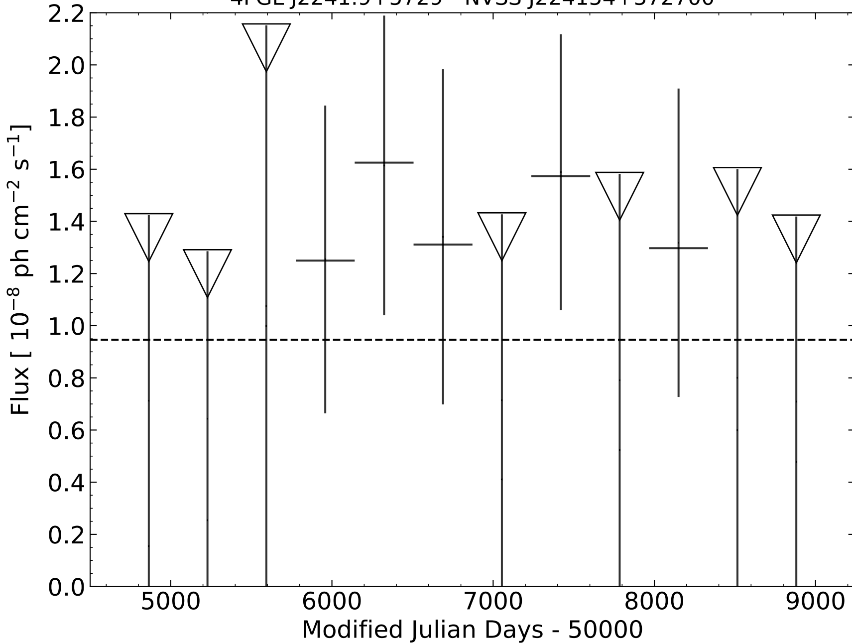
4FGL J2241.9+5729 - NVSS J224154+572700
