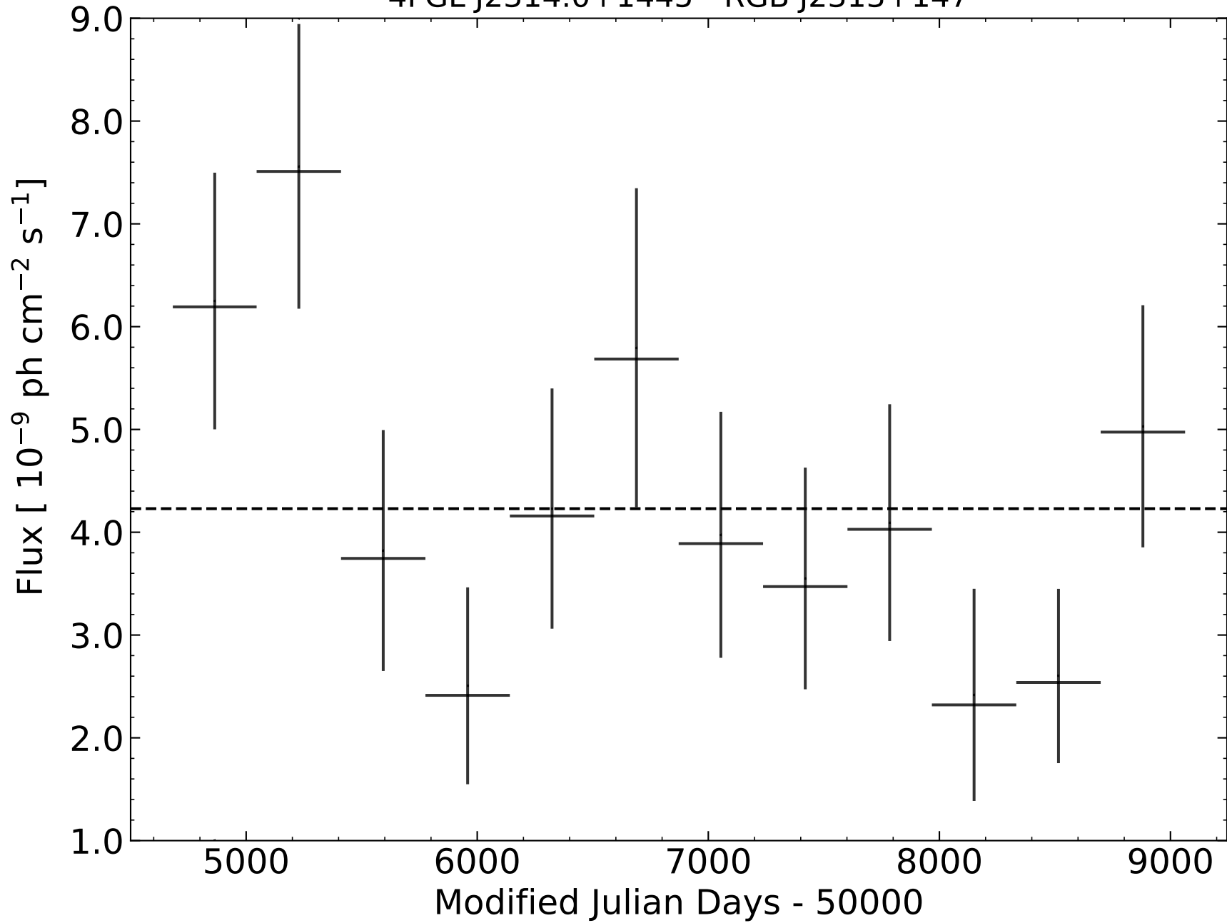
4FGL J2314.0+1445 - RGB J2313+147
