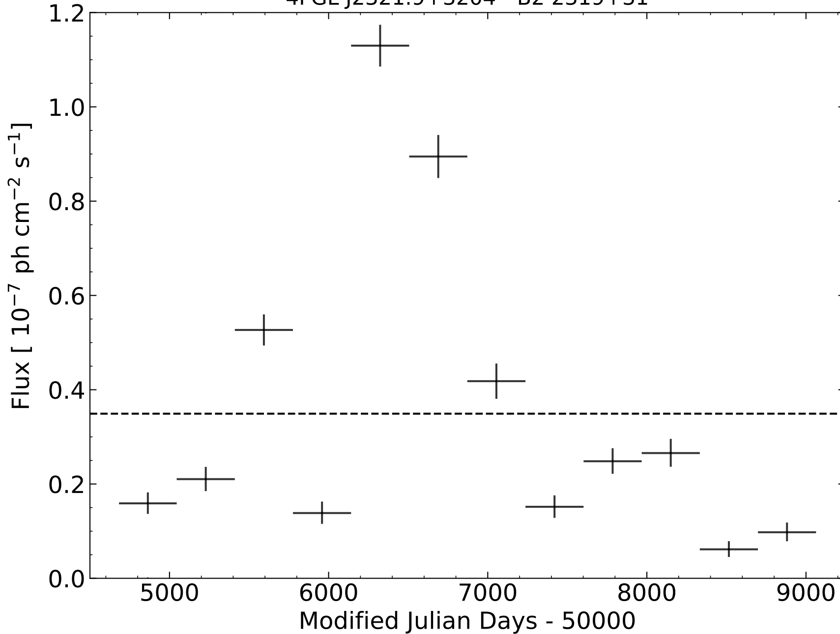
4FGL J2321.9+3204 - B2 2319+31
