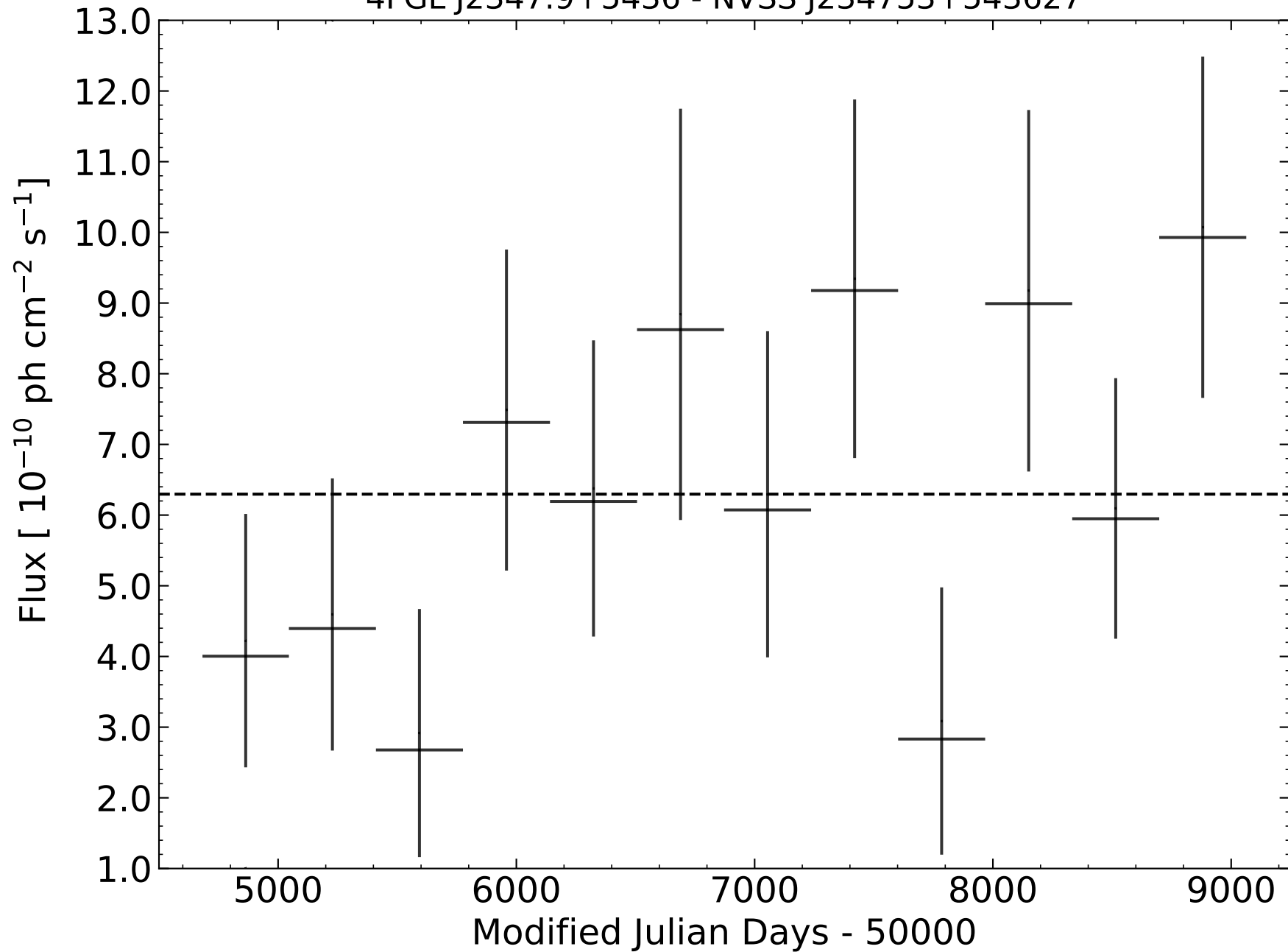
4FGL J2347.9+5436 - NVSS J234753+543627
