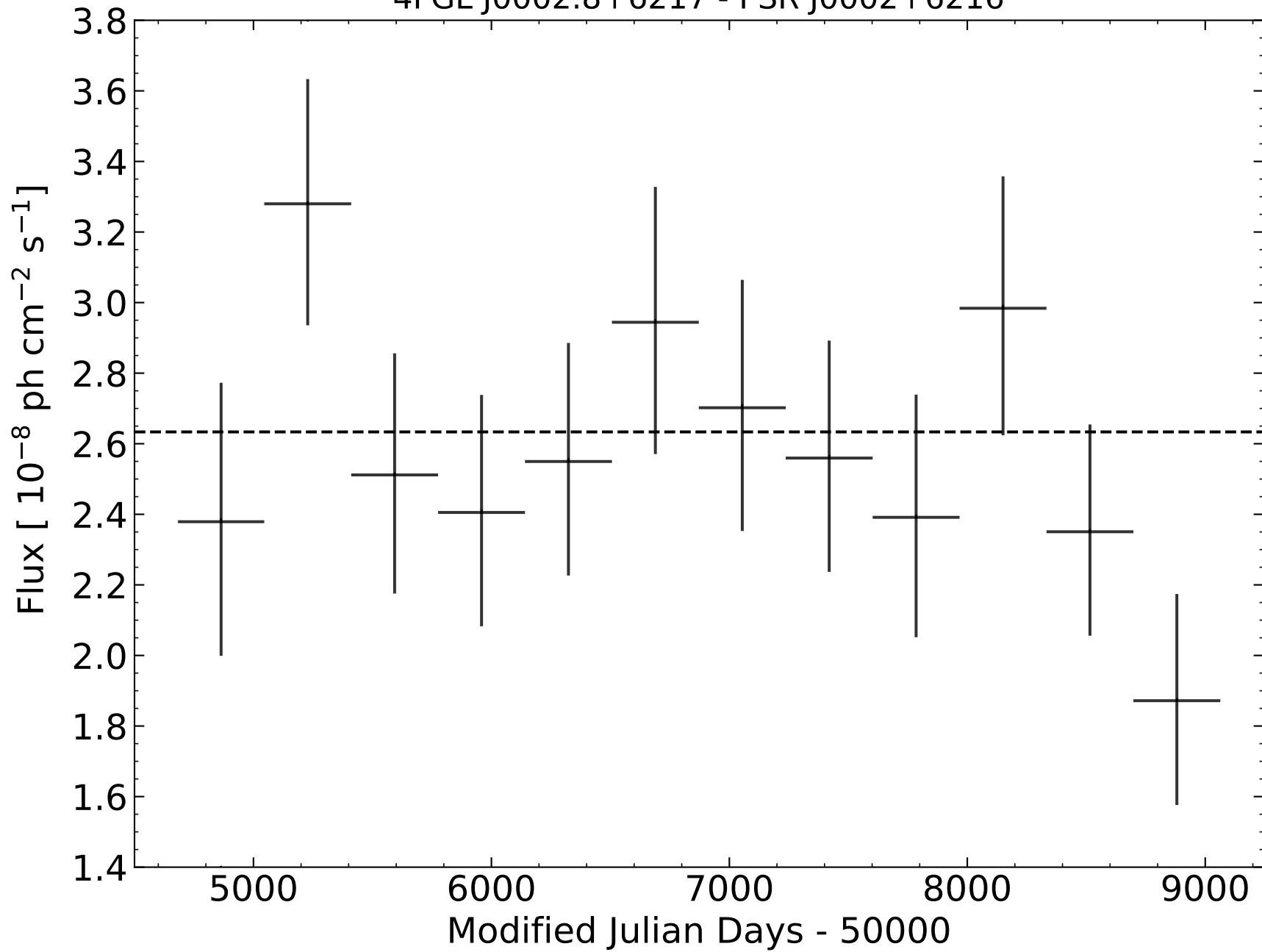
4FGL J0002.8+6217 - PSR J0002+6216
