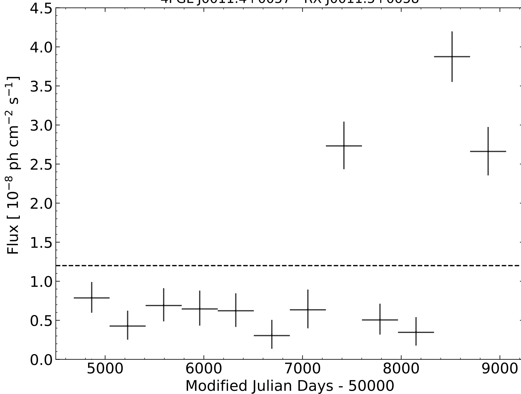
4FGL J0011.4+0057 - RX J0011.5+0058
