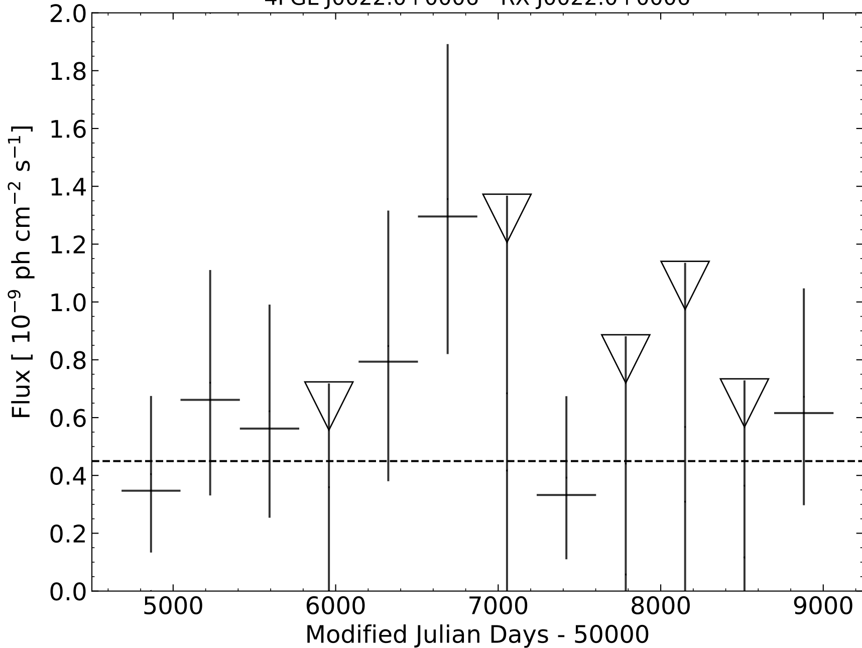
4FGL J0022.0+0006 - RX J0022.0+0006
