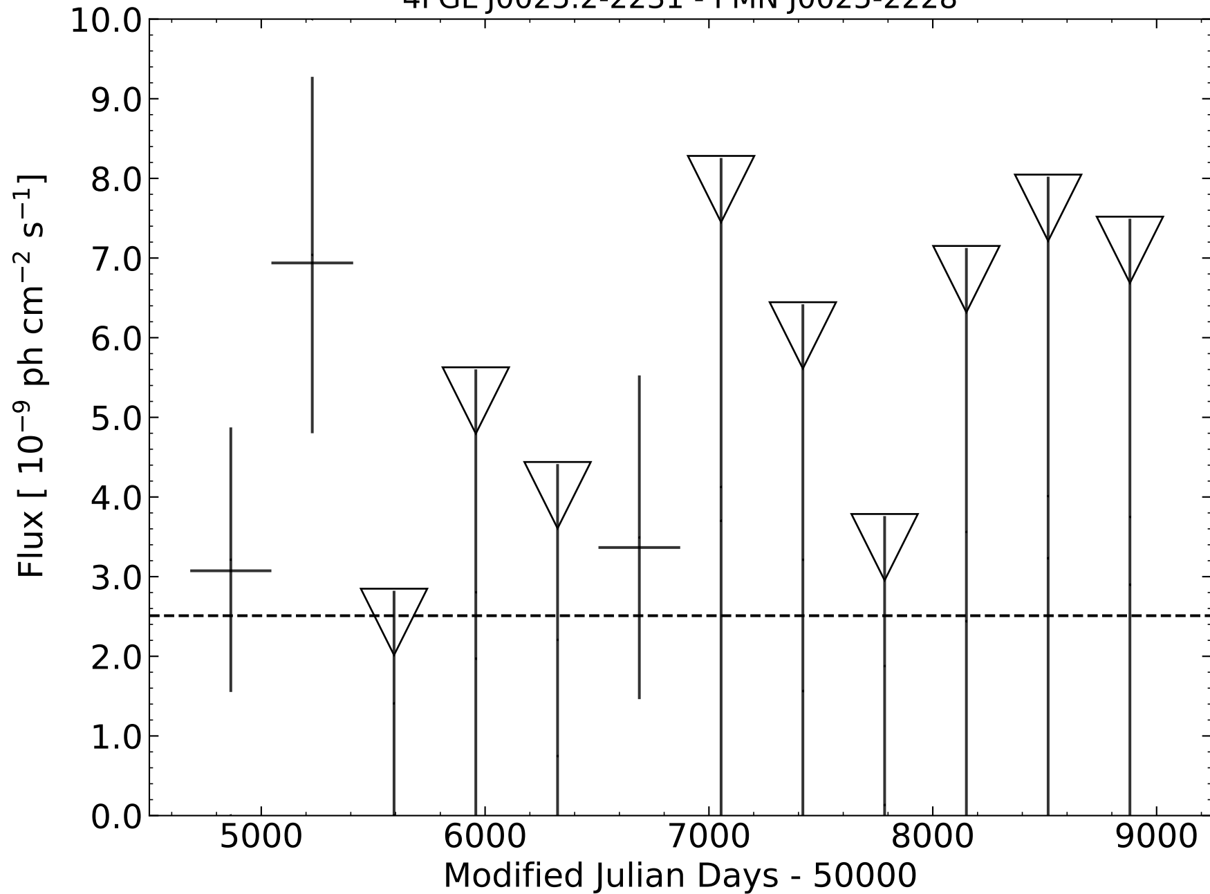
4FGL J0025.2-2231 - PMN J0025-2228
