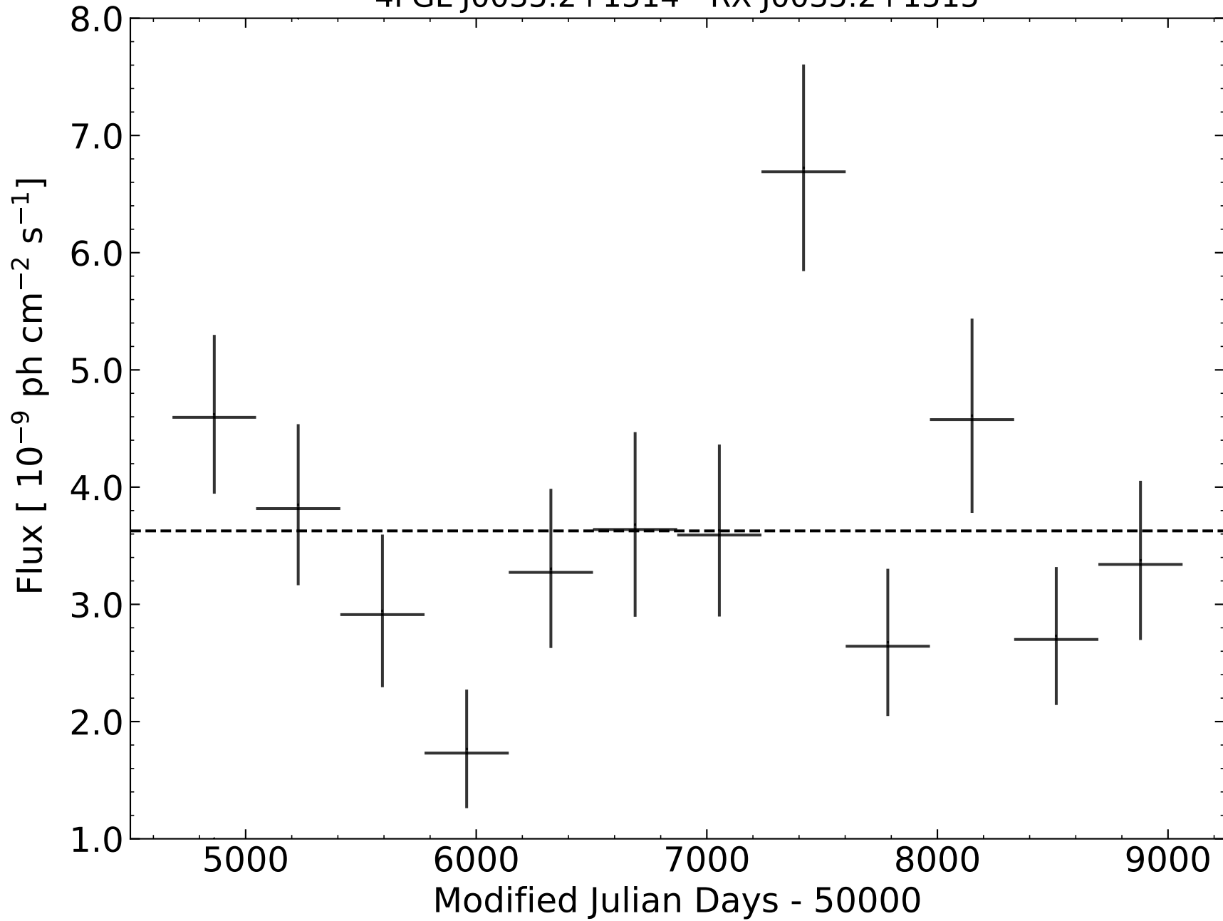
4FGL J0035.2+1514 - RX J0035.2+1515
