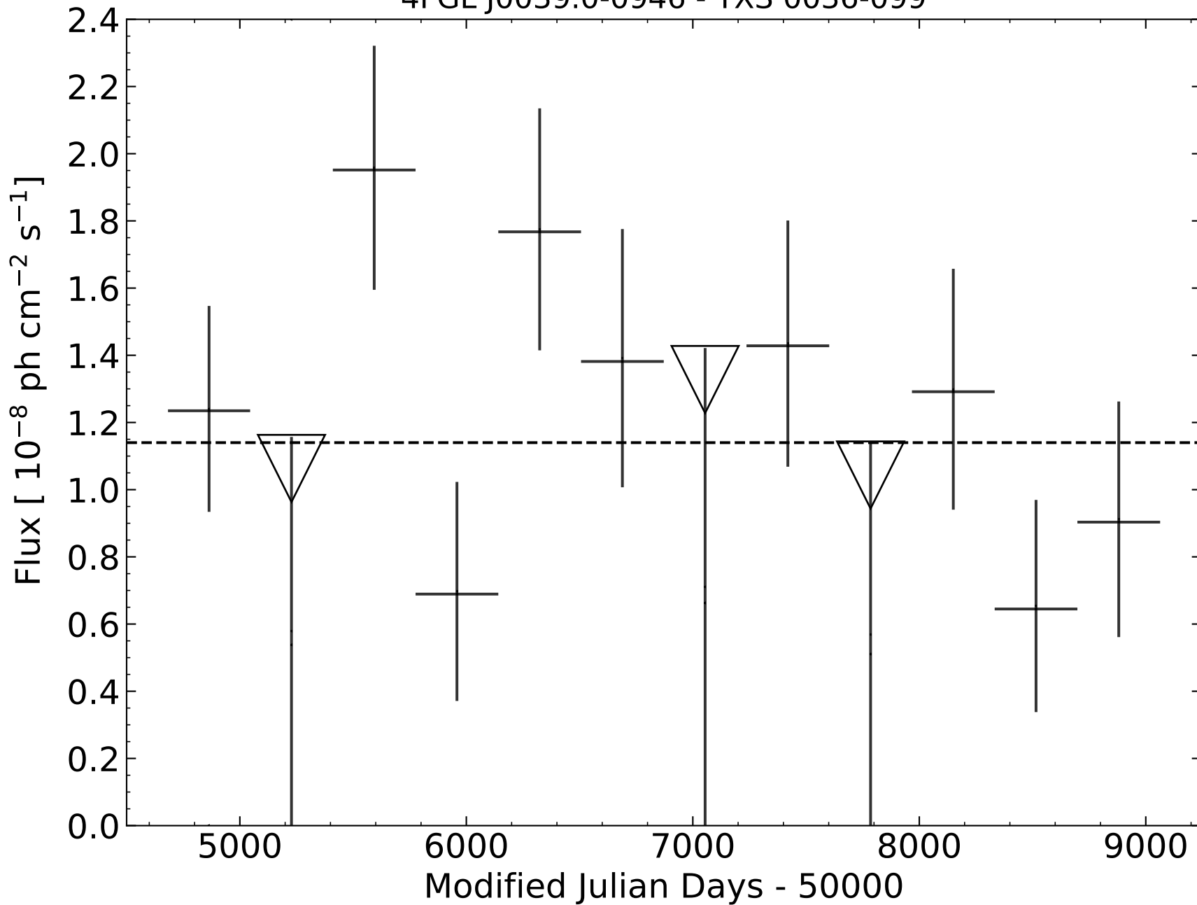
4FGL J0039.0-0946 - TXS 0036-099
