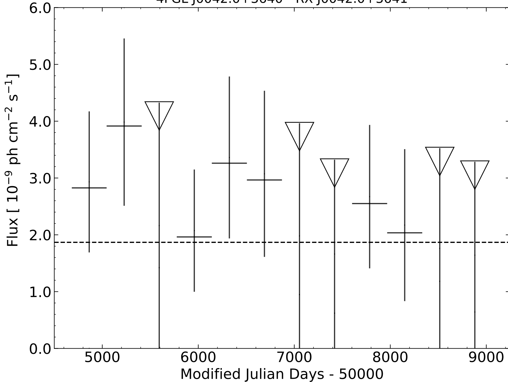
4FGL J0042.0+3640 - RX J0042.0+3641
