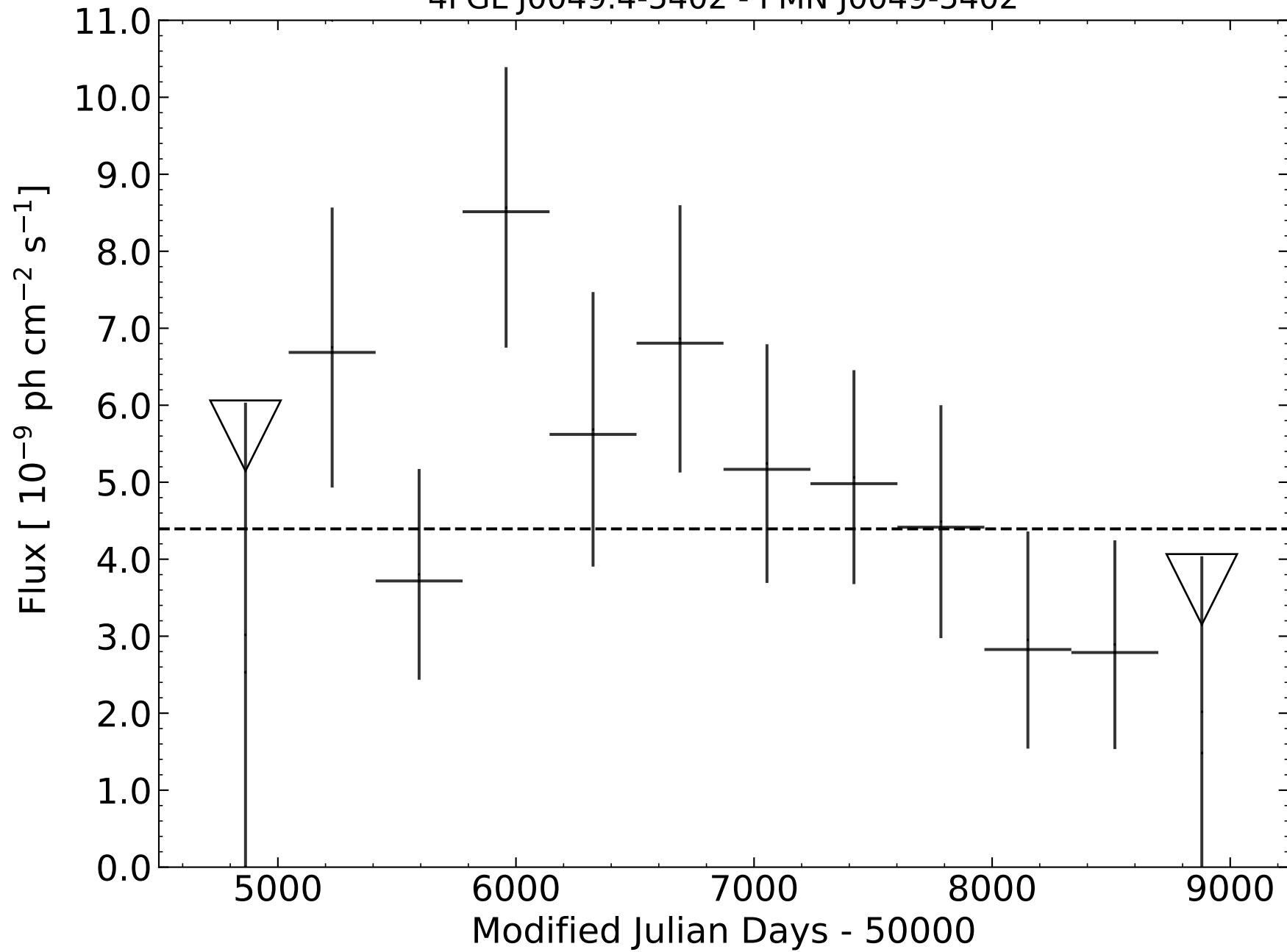
4FGL J0049.4-5402 - PMN J0049-5402
