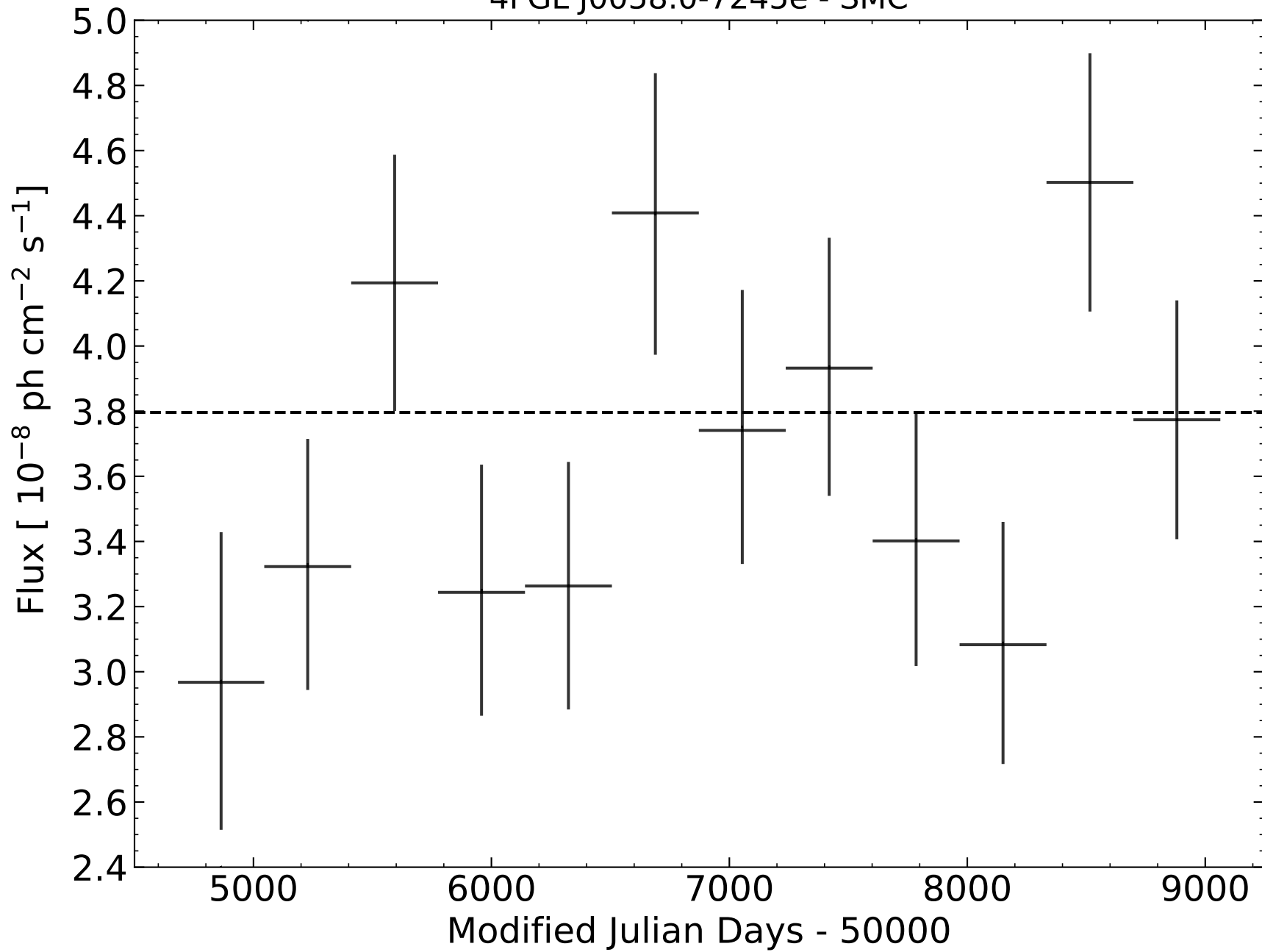
4FGL J0058.0-7245e - SMC
