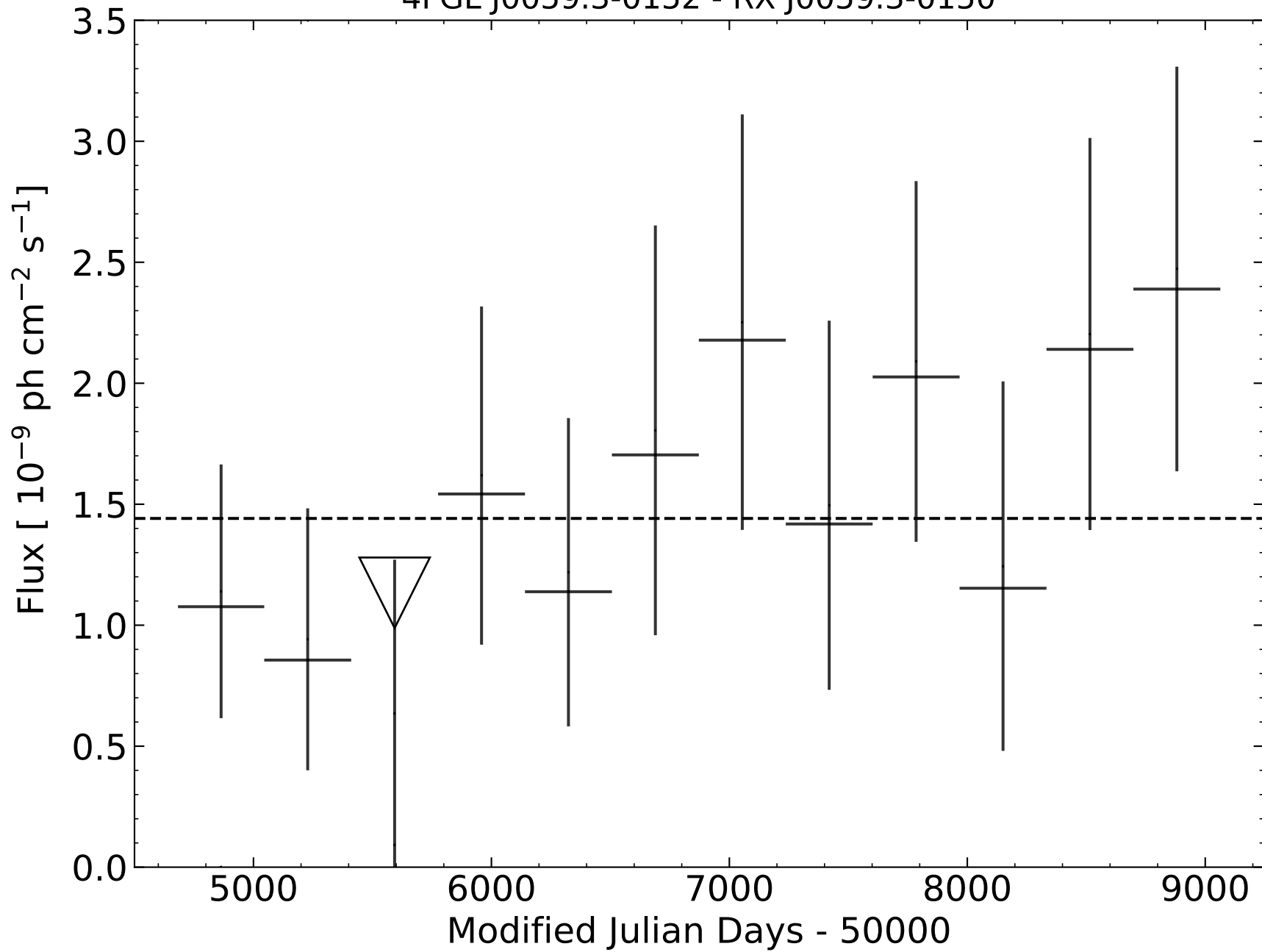
4FGL J0059.3-0152 - RX J0059.3-0150
