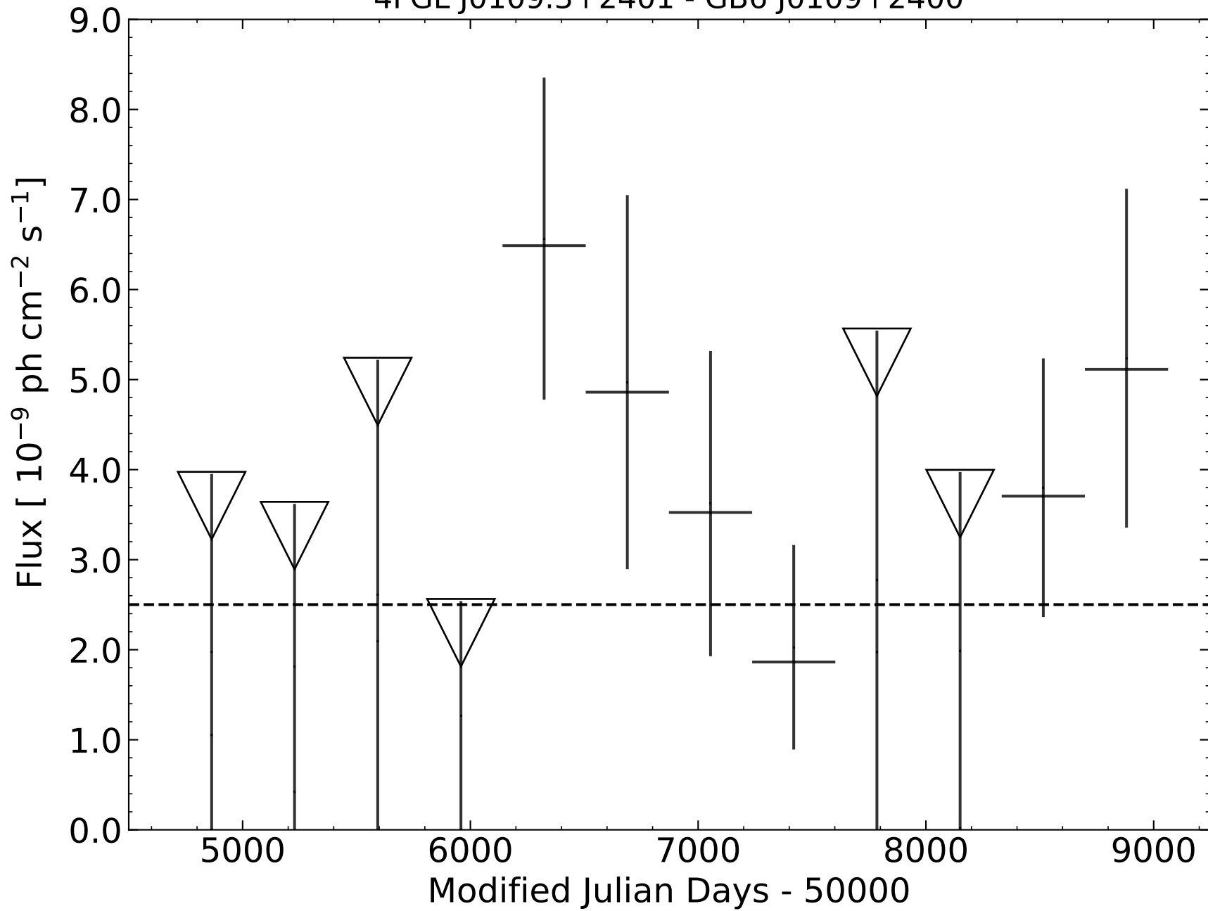
4FGL J0109.3+2401 - GB6 J0109+2400
