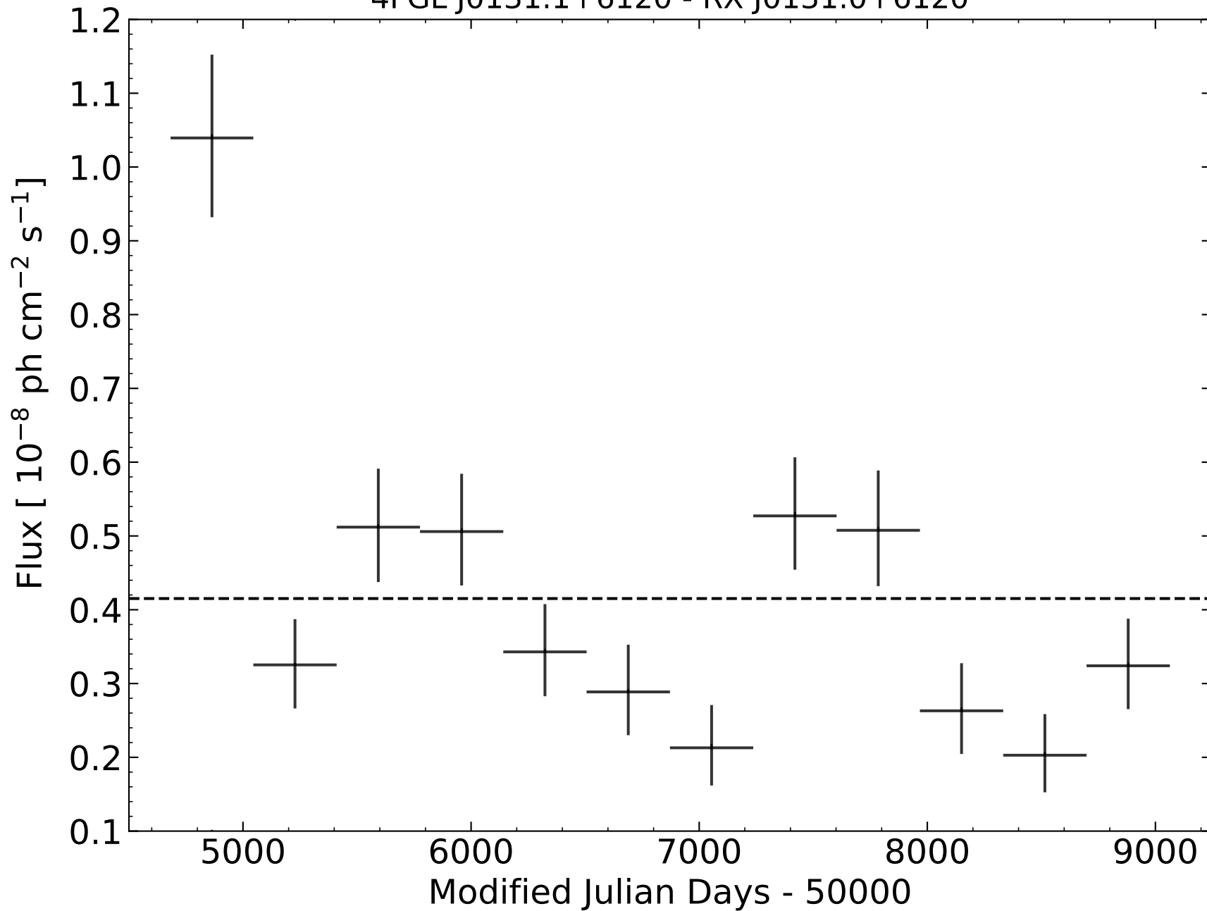
4FGL J0131.1+6120 - RX J0131.0+6120
