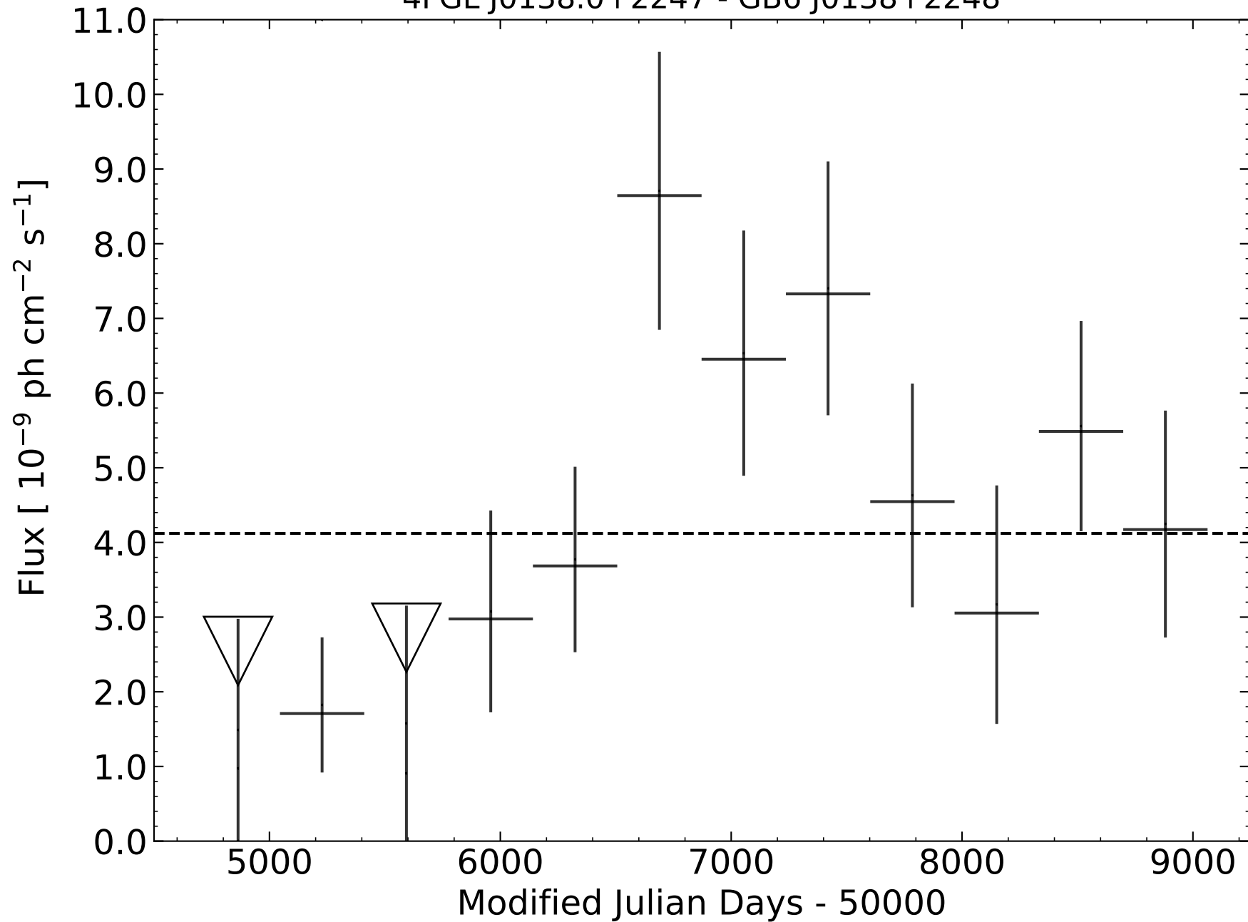
4FGL J0138.0+2247 - GB6 J0138+2248
