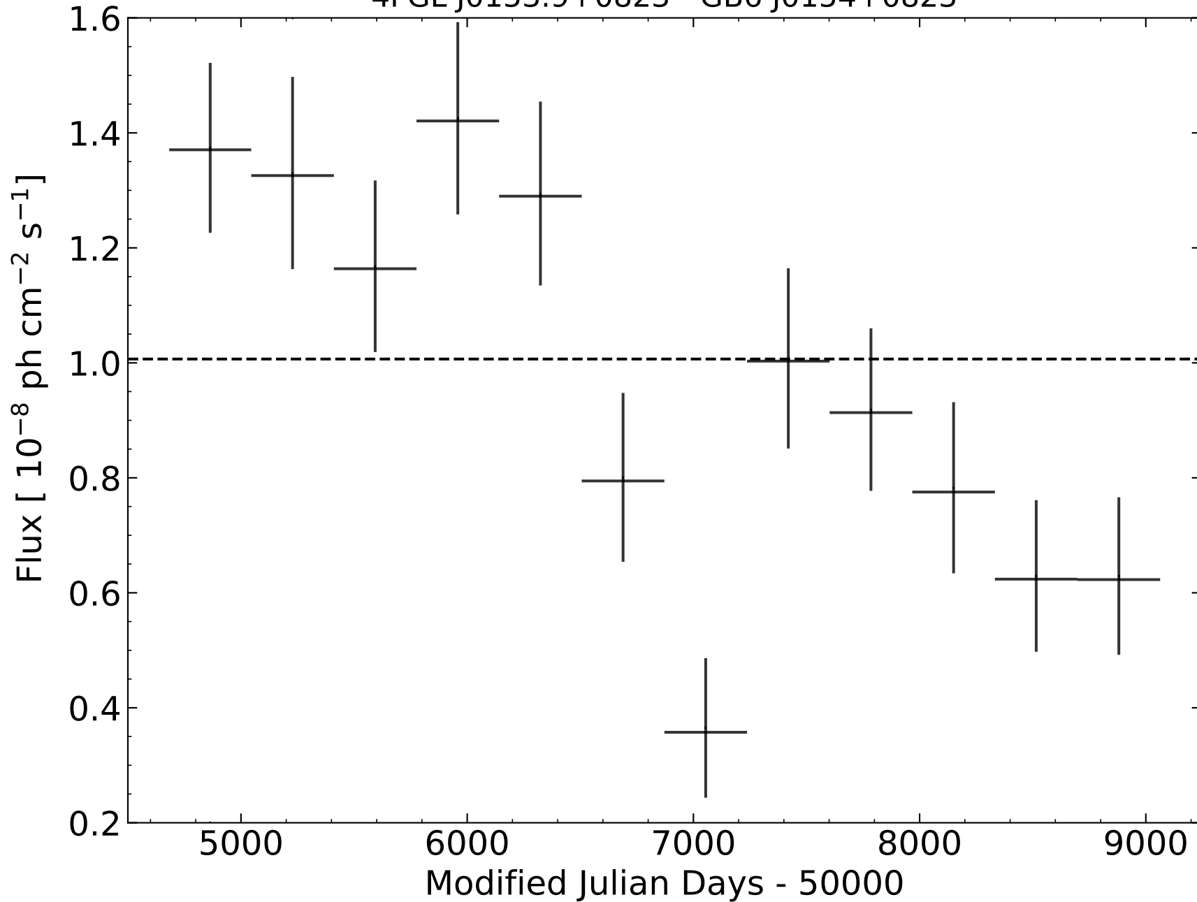
4FGL J0153.9+0823 - GB6 J0154+0823
