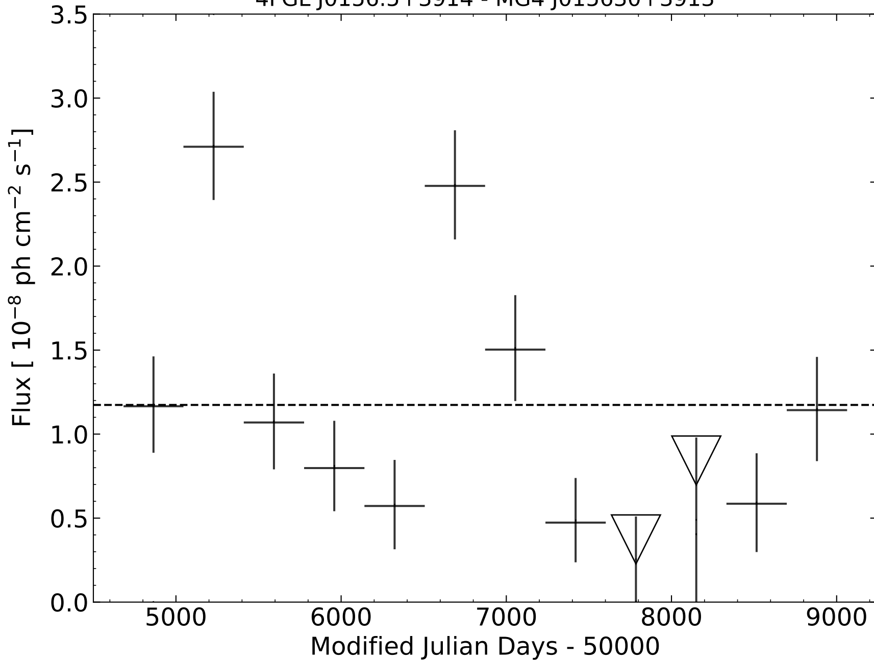
4FGL J0156.5+3914 - MG4 J015630+3913
