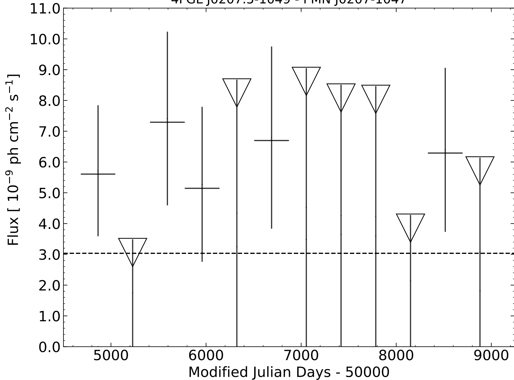
4FGL J0207.5-1049 - PMN J0207-1047
