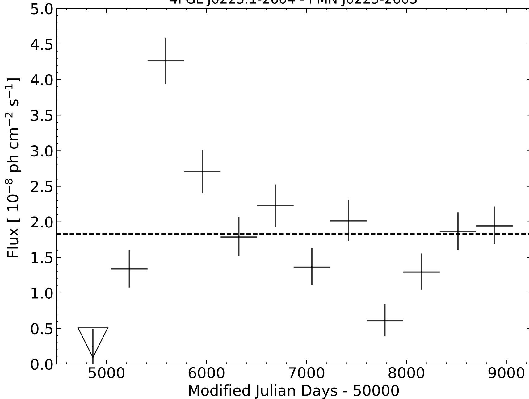
4FGL J0225.1-2604 - PMN J0225-2603
