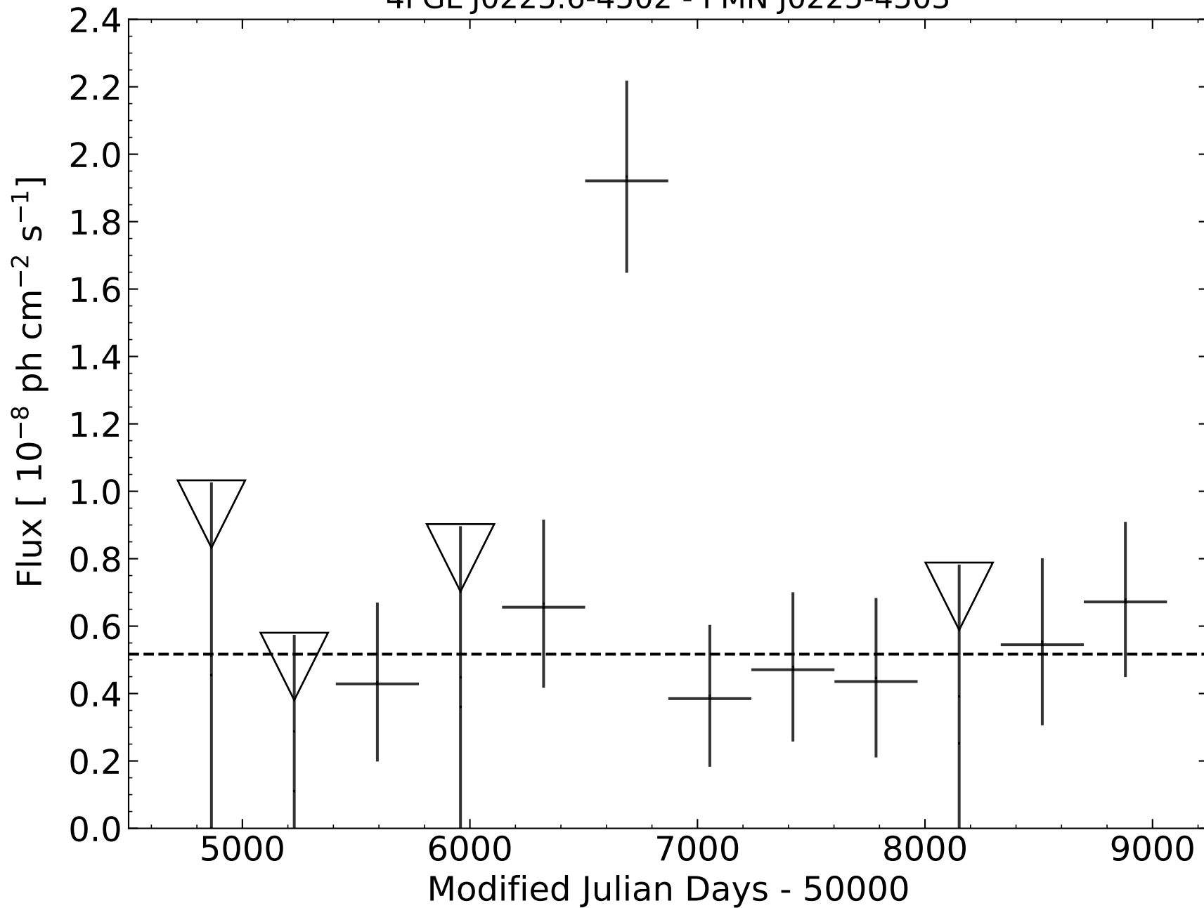
4FGL J0225.6-4502 - PMN J0225-4503
