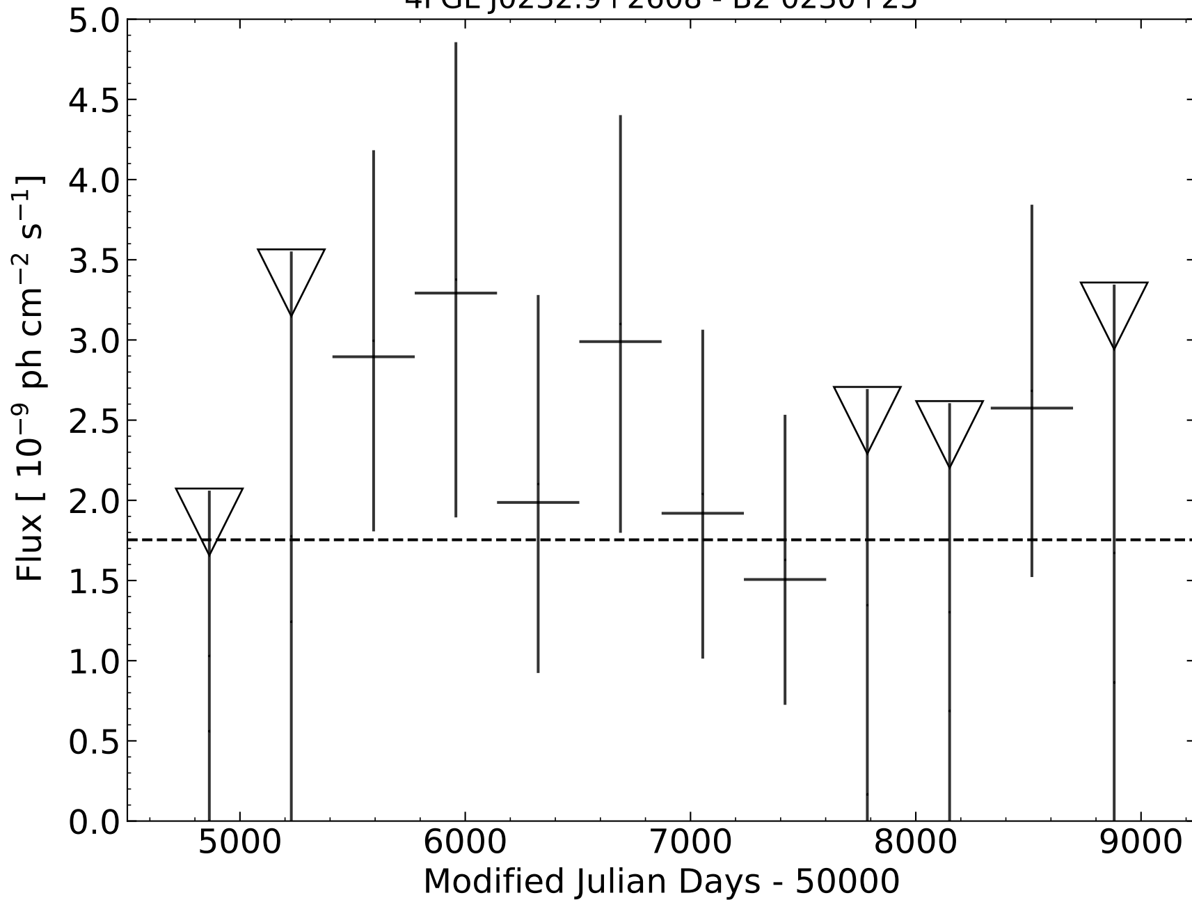
4FGL J0232.9+2608 - B2 0230+25
