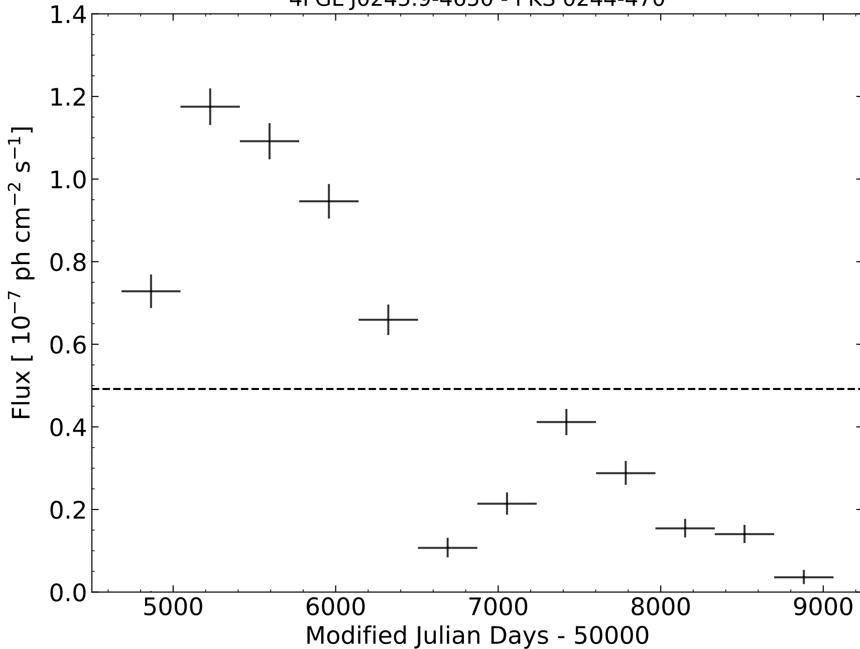
4FGL J0245.9-4650 - PKS 0244-470
