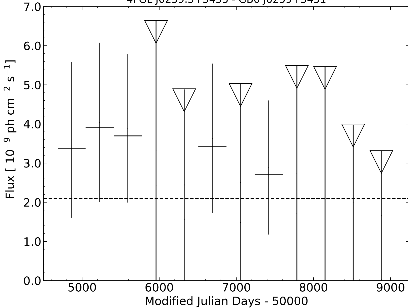
4FGL J0259.3+5453 - GB6 J0259+5451
