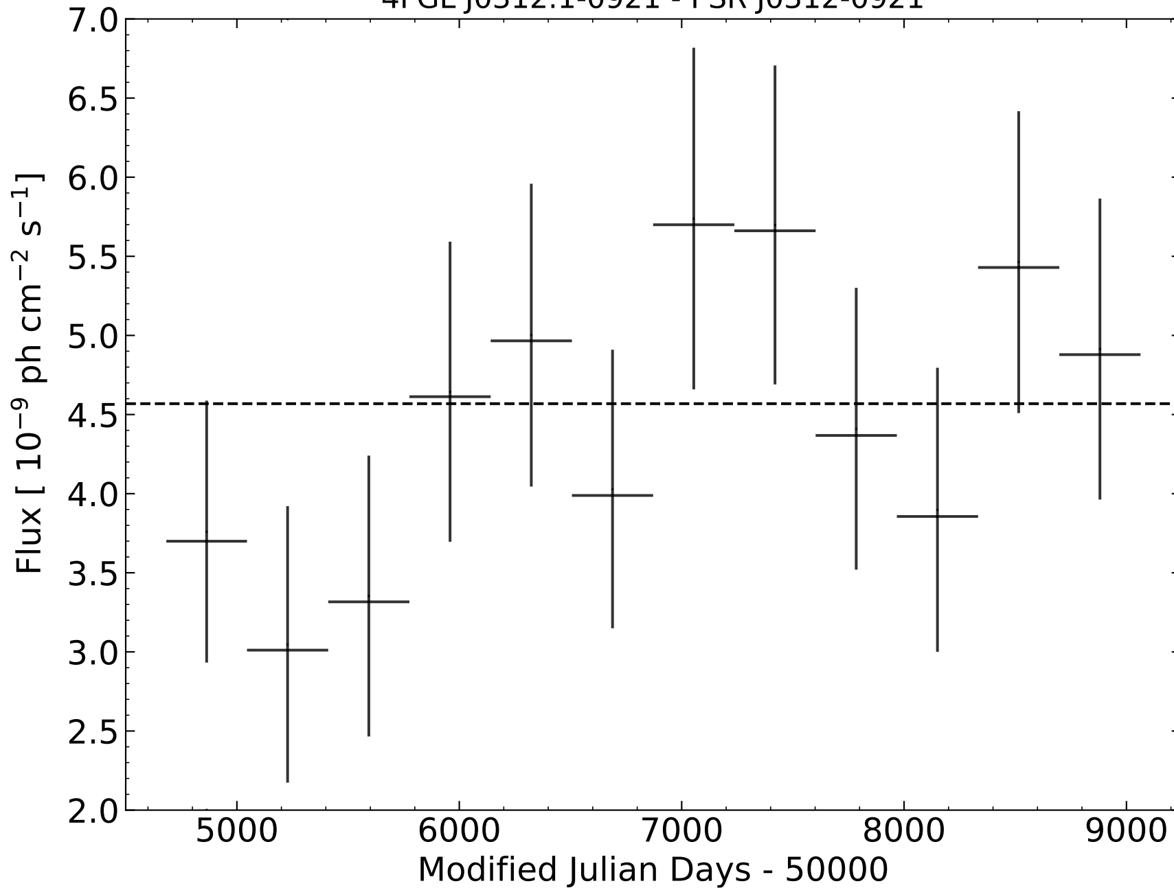
4FGL J0312.1-0921 - PSR J0312-0921
