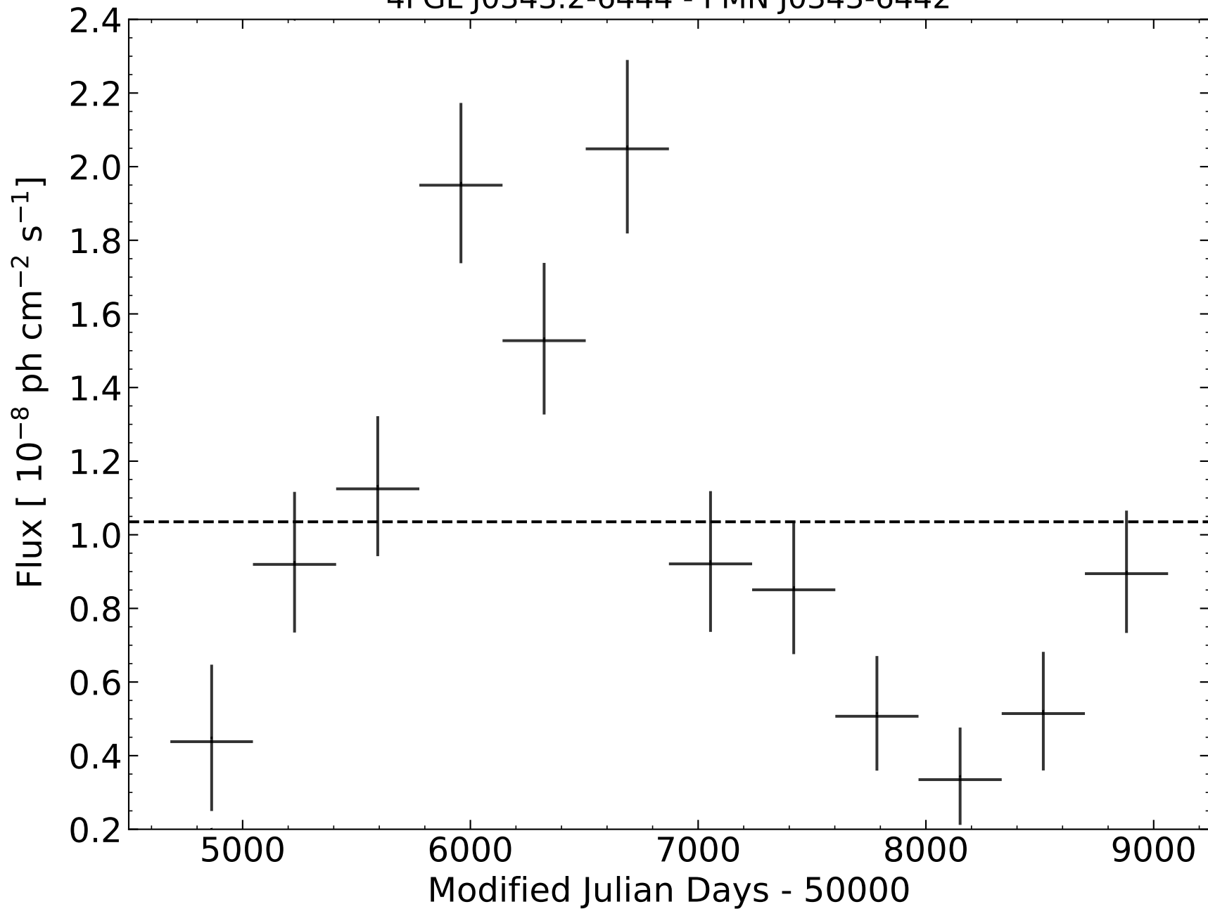
4FGL J0343.2-6444 - PMN J0343-6442
