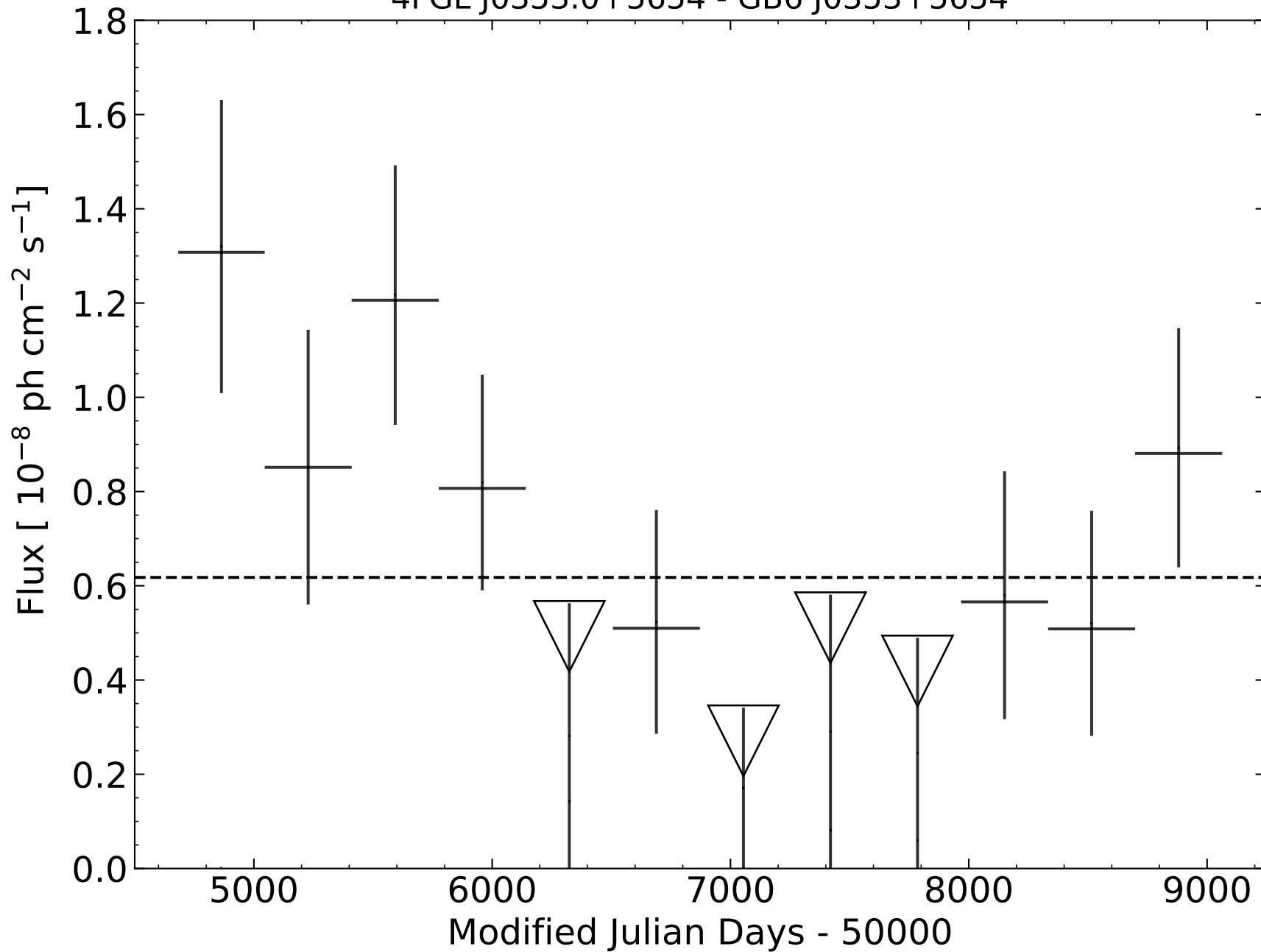
4FGL J0353.0+5654 - GB6 J0353+5654
