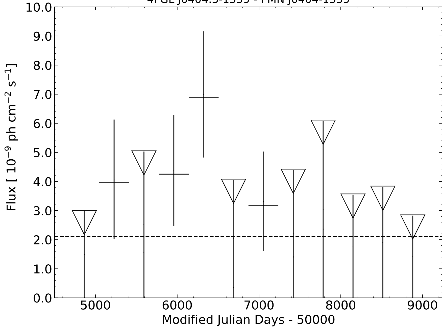
4FGL J0404.3-1559 - PMN J0404-1559
