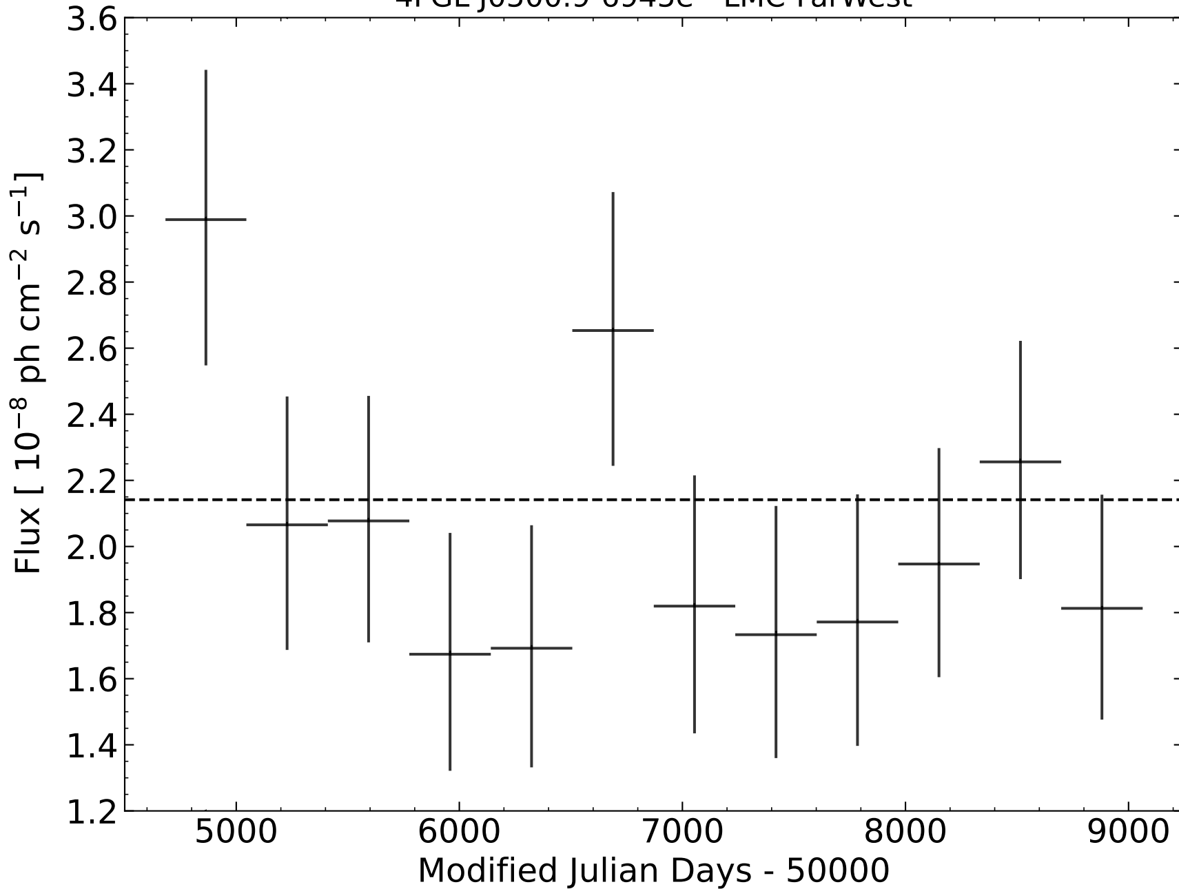
4FGL J0500.9-6945e - LMC-FarWest
