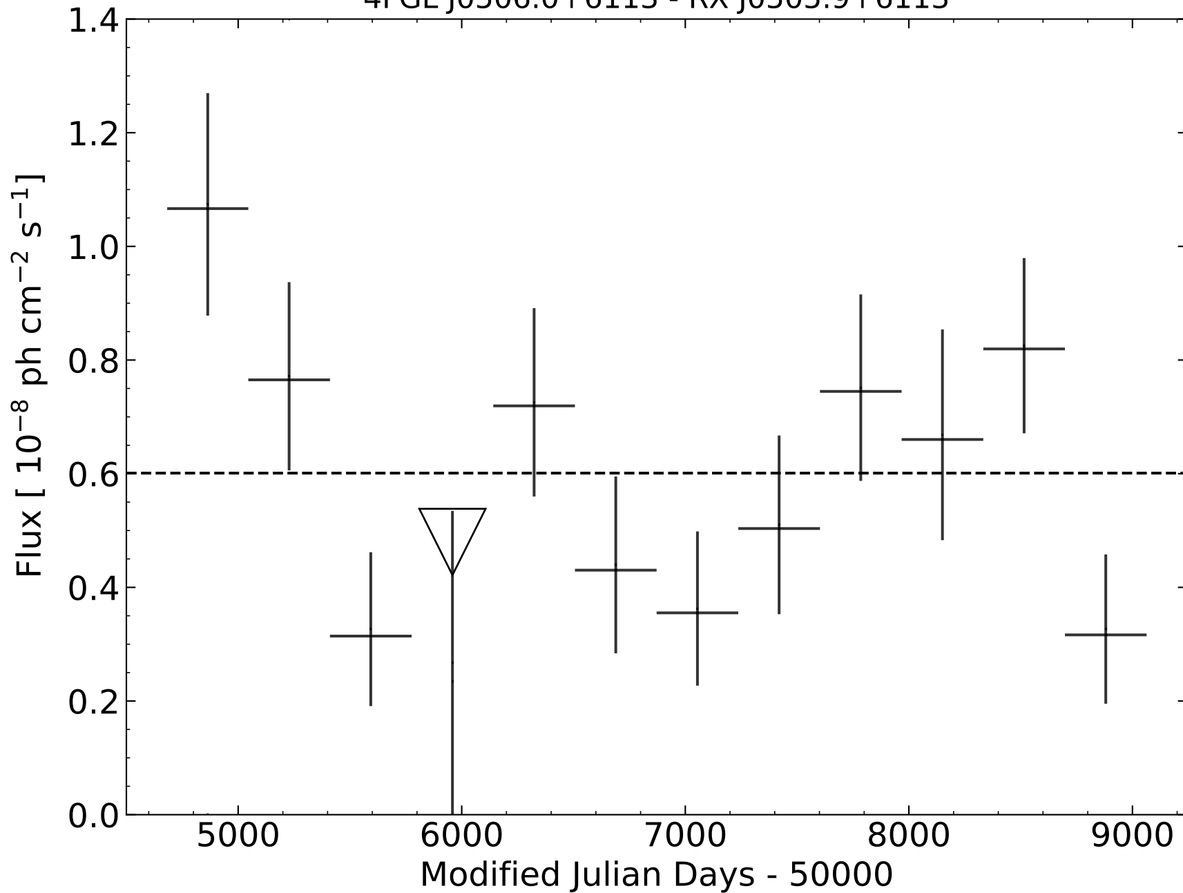
4FGL J0506.0+6113 - RX J0505.9+6113
