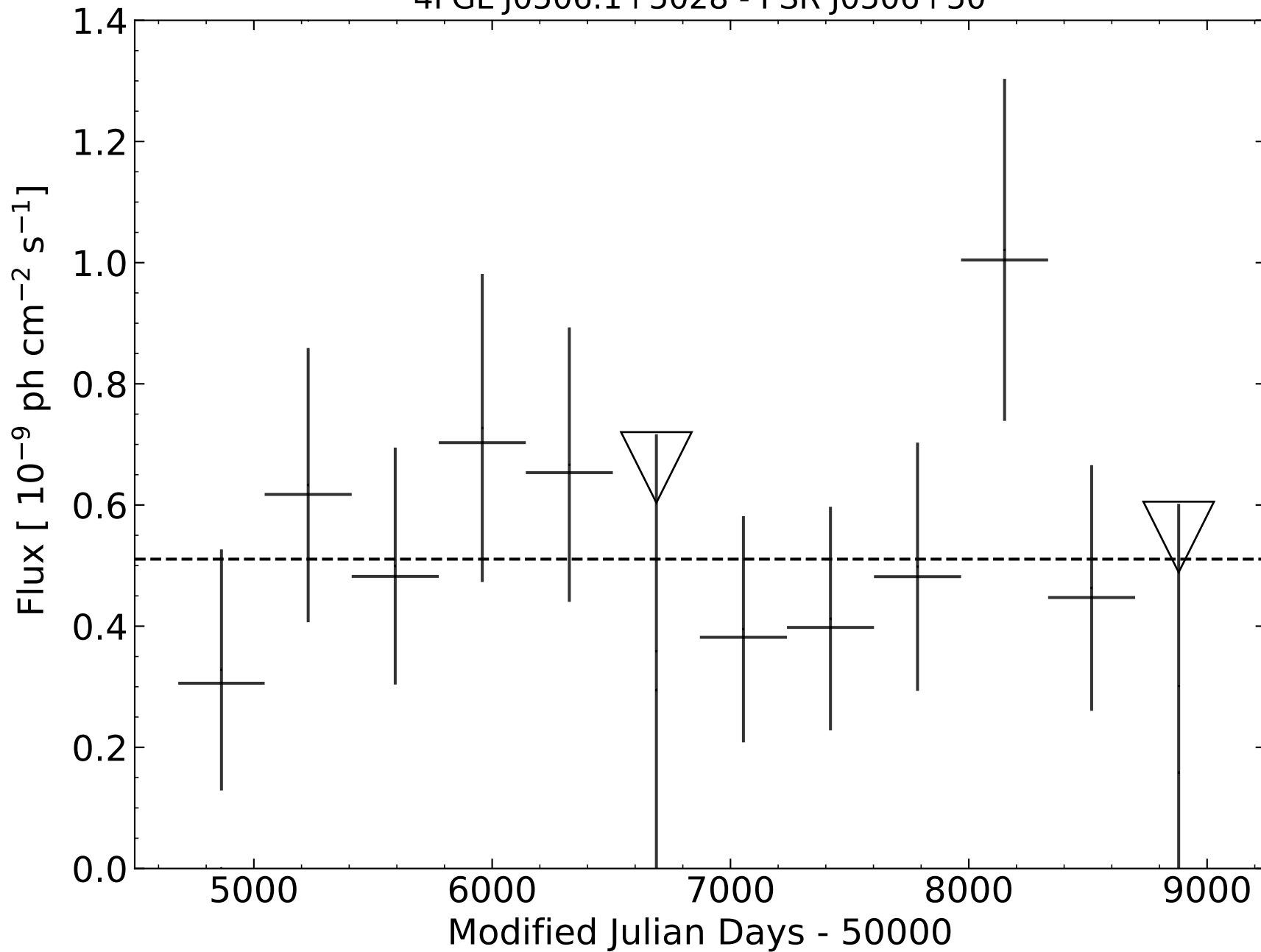
4FGL J0506.1+5028 - PSR J0506+50
