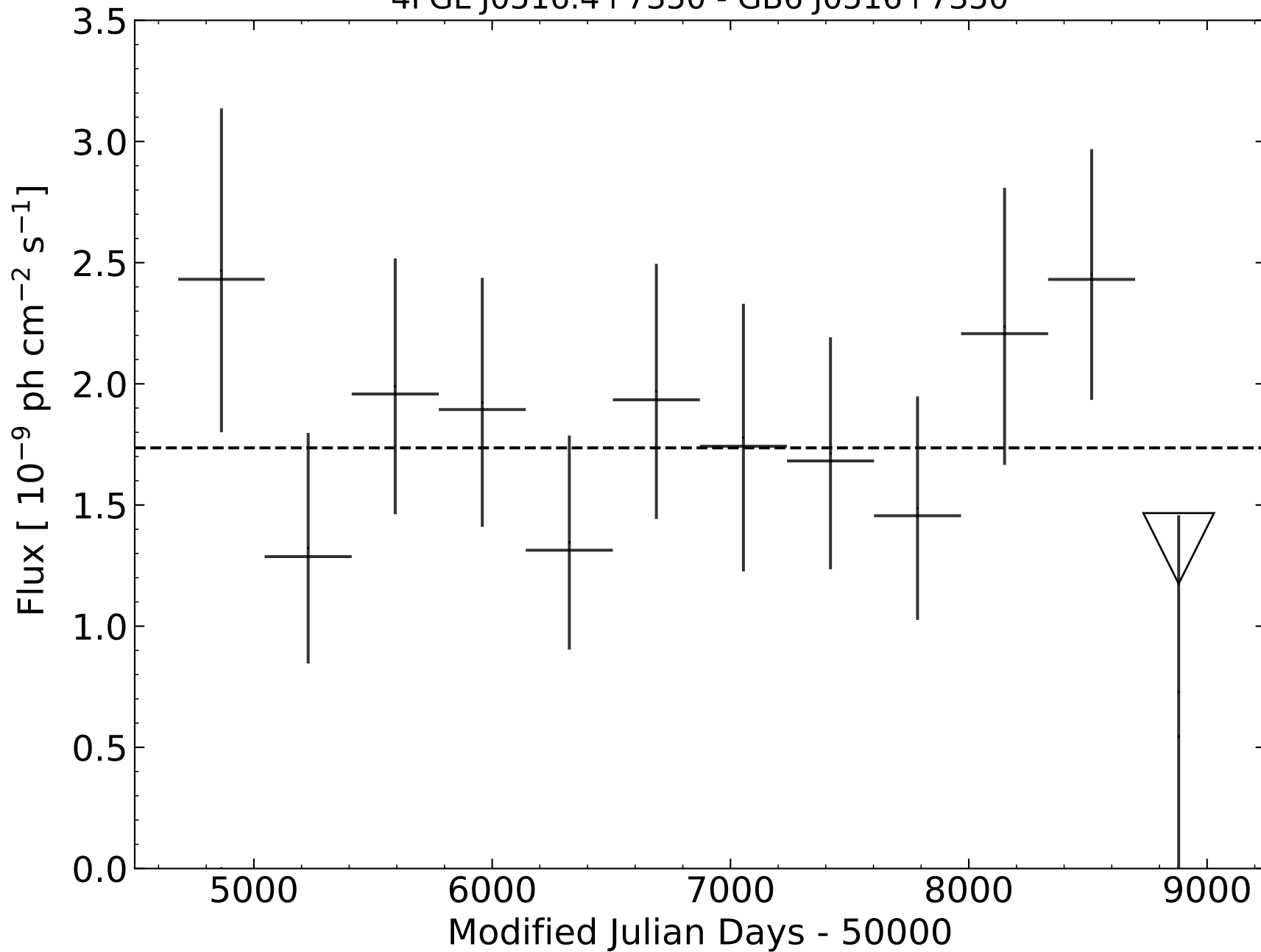
4FGL J0516.4+7350 - GB6 J0516+7350
