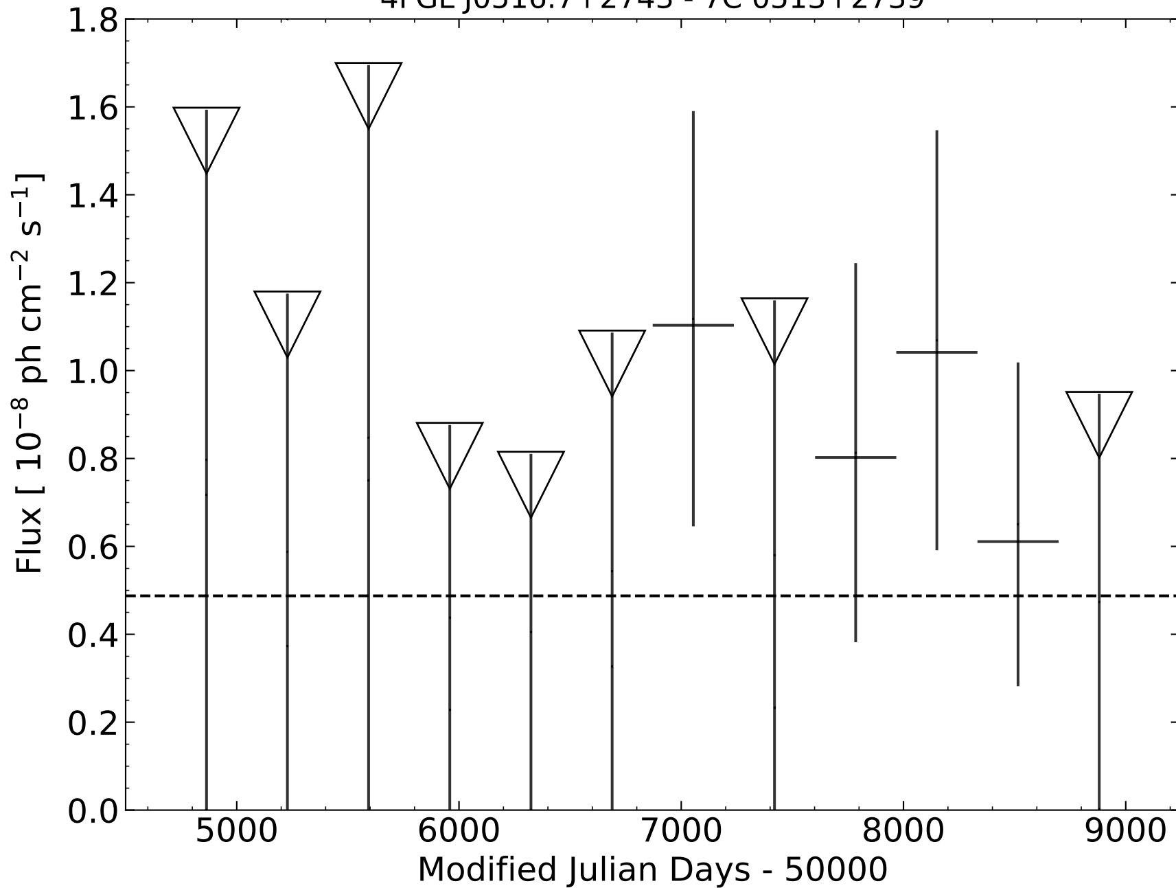
4FGL J0516.7+2743 - 7C 0513+2739
