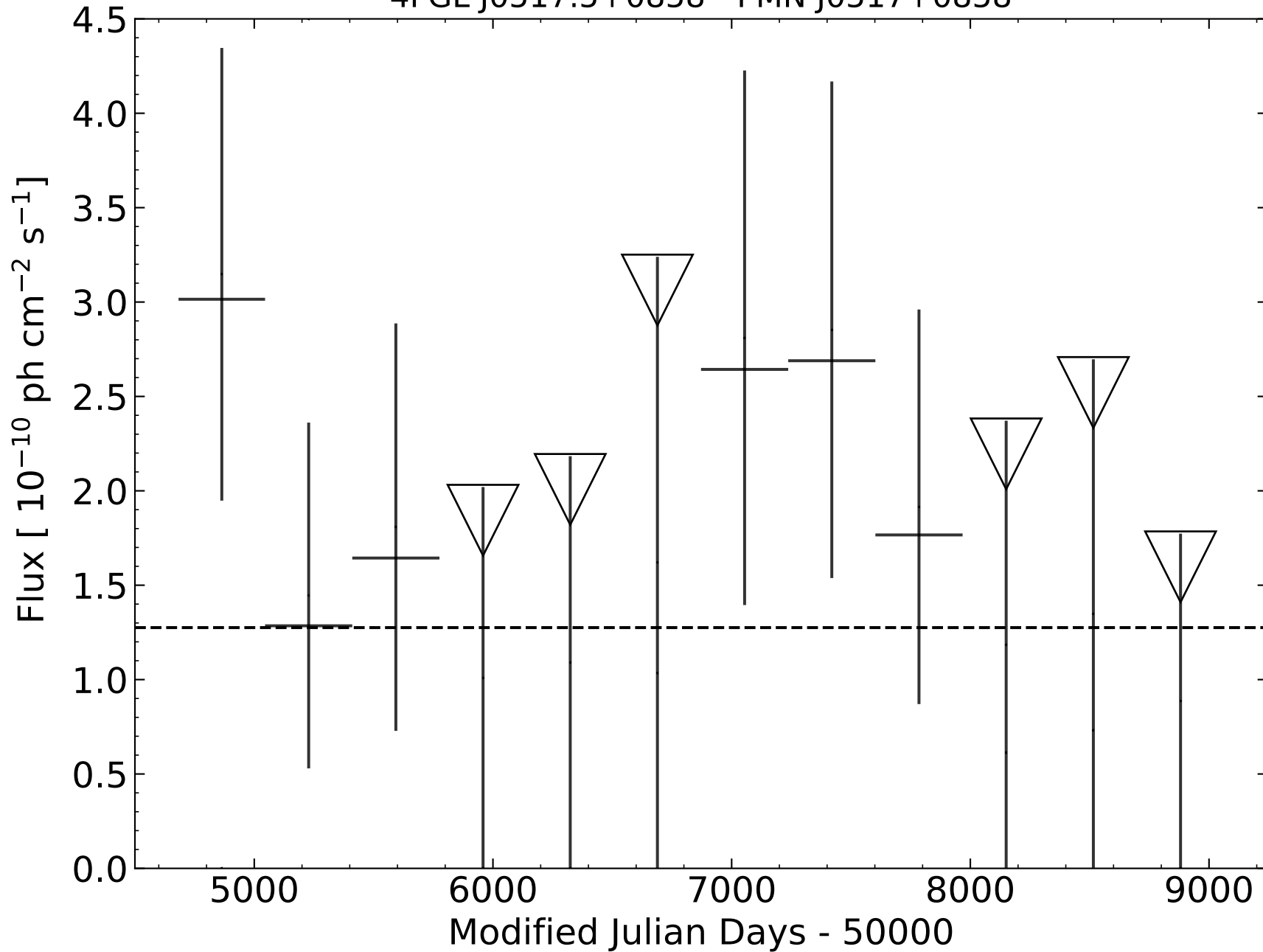
4FGL J0517.5+0858 - PMN J0517+0858
