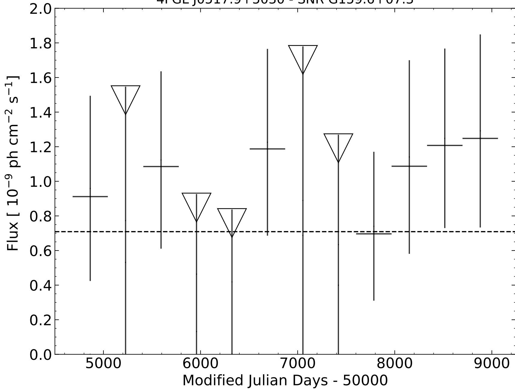
4FGL J0517.9+5030 - SNR G159.6+07.3
